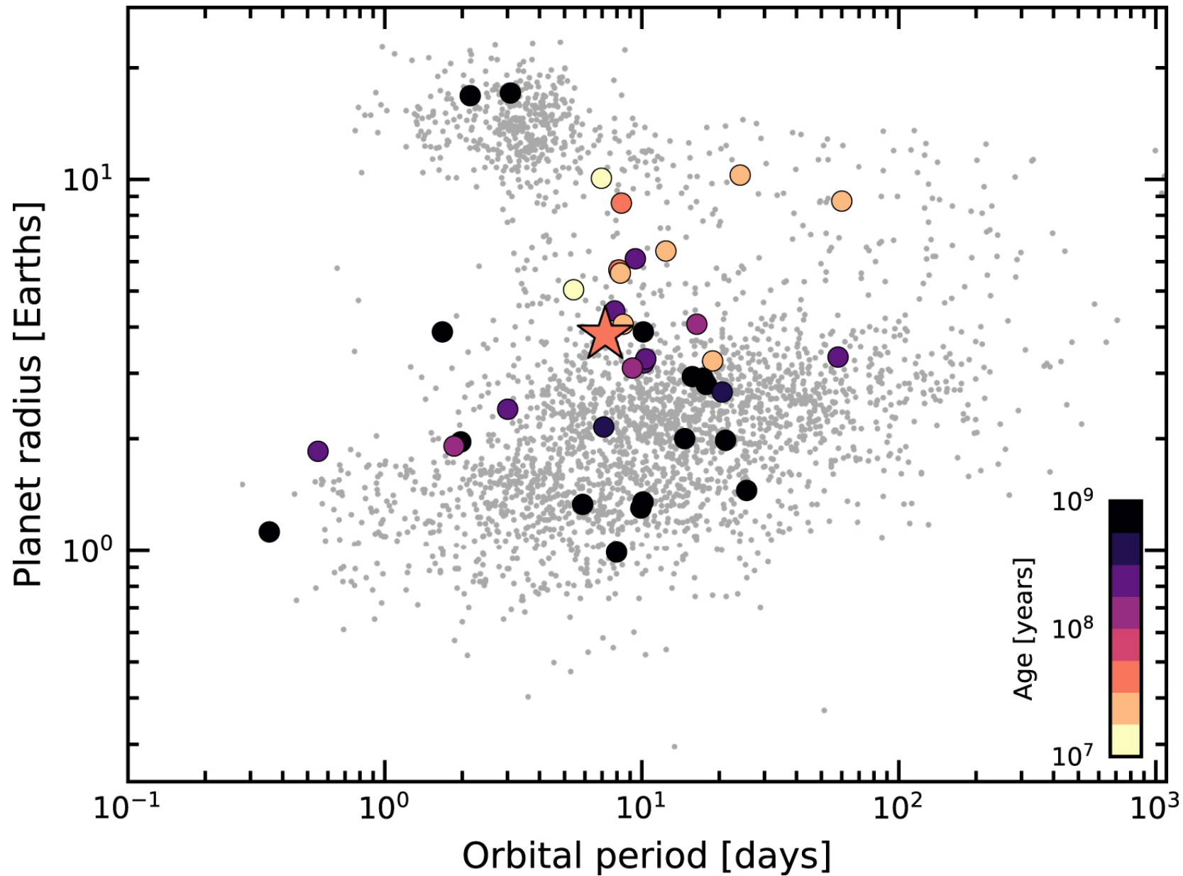
Figure 9. from L. G. Bouma et al 2022 Astron. J. 163 doi:10.3847/1538-3881/ac4966 https://dx.doi.org/10.3847/1538-3881/ac4966 © 2022. The Author(s). Published by the American Astronomical Society.
