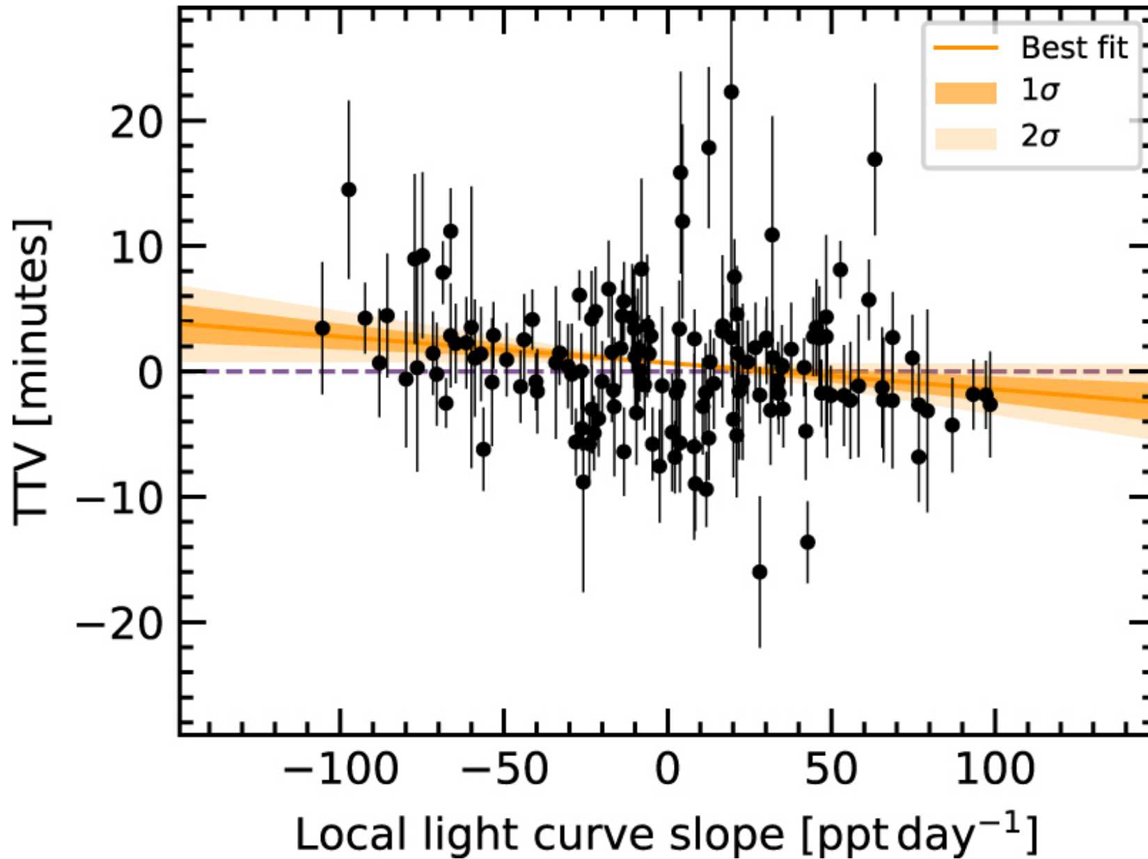
Figure 7. from L. G. Bouma et al 2022 Astron. J. 163 doi:10.3847/1538-3881/ac4966 https://dx.doi.org/10.3847/1538-3881/ac4966 © 2022. The Author(s). Published by the American Astronomical Society.
