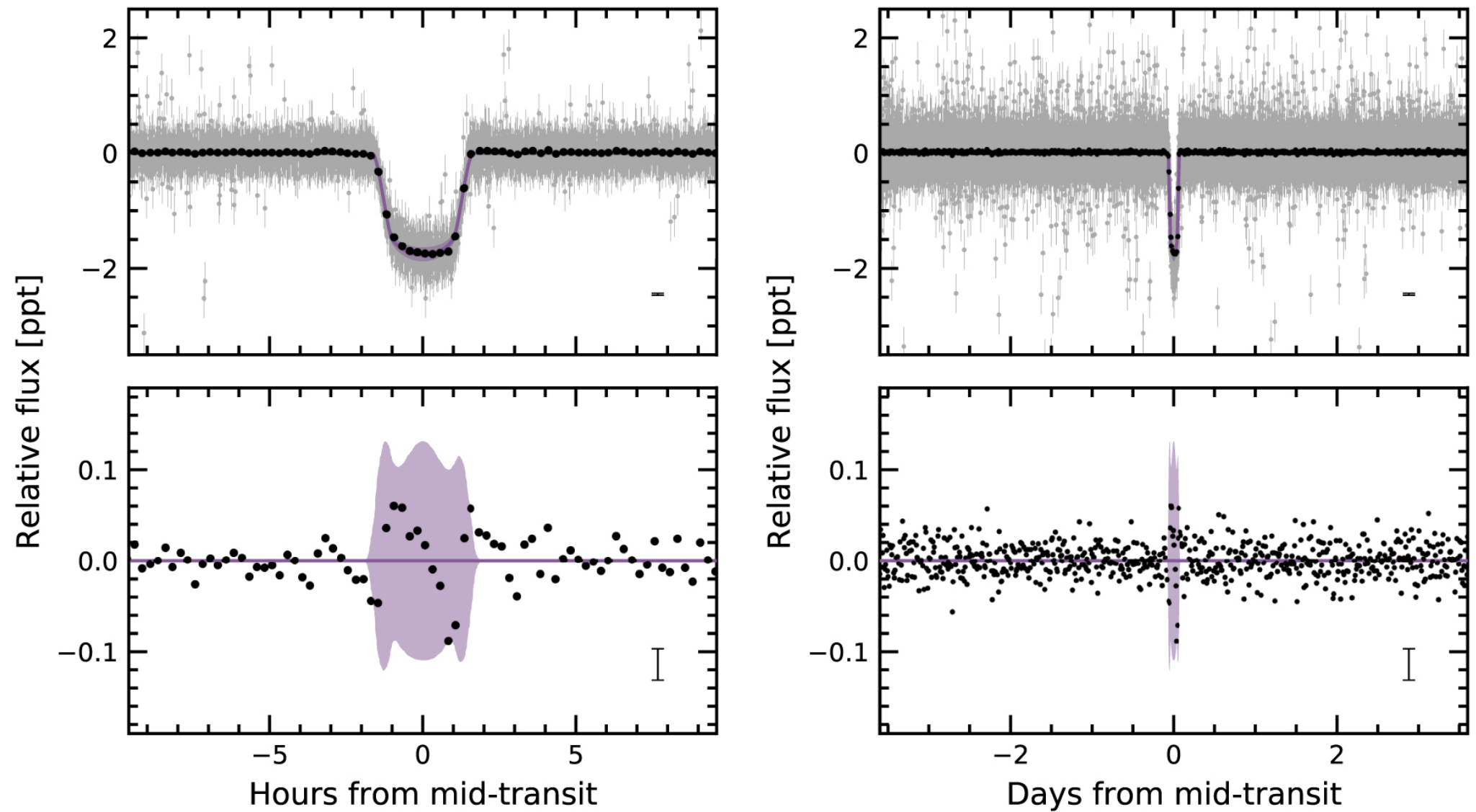
Figure 6. from L. G. Bouma et al 2022 Astron. J. 163 doi:10.3847/1538-3881/ac4966 https://dx.doi.org/10.3847/1538-3881/ac4966 © 2022. The Author(s). Published by the American Astronomical Society.
