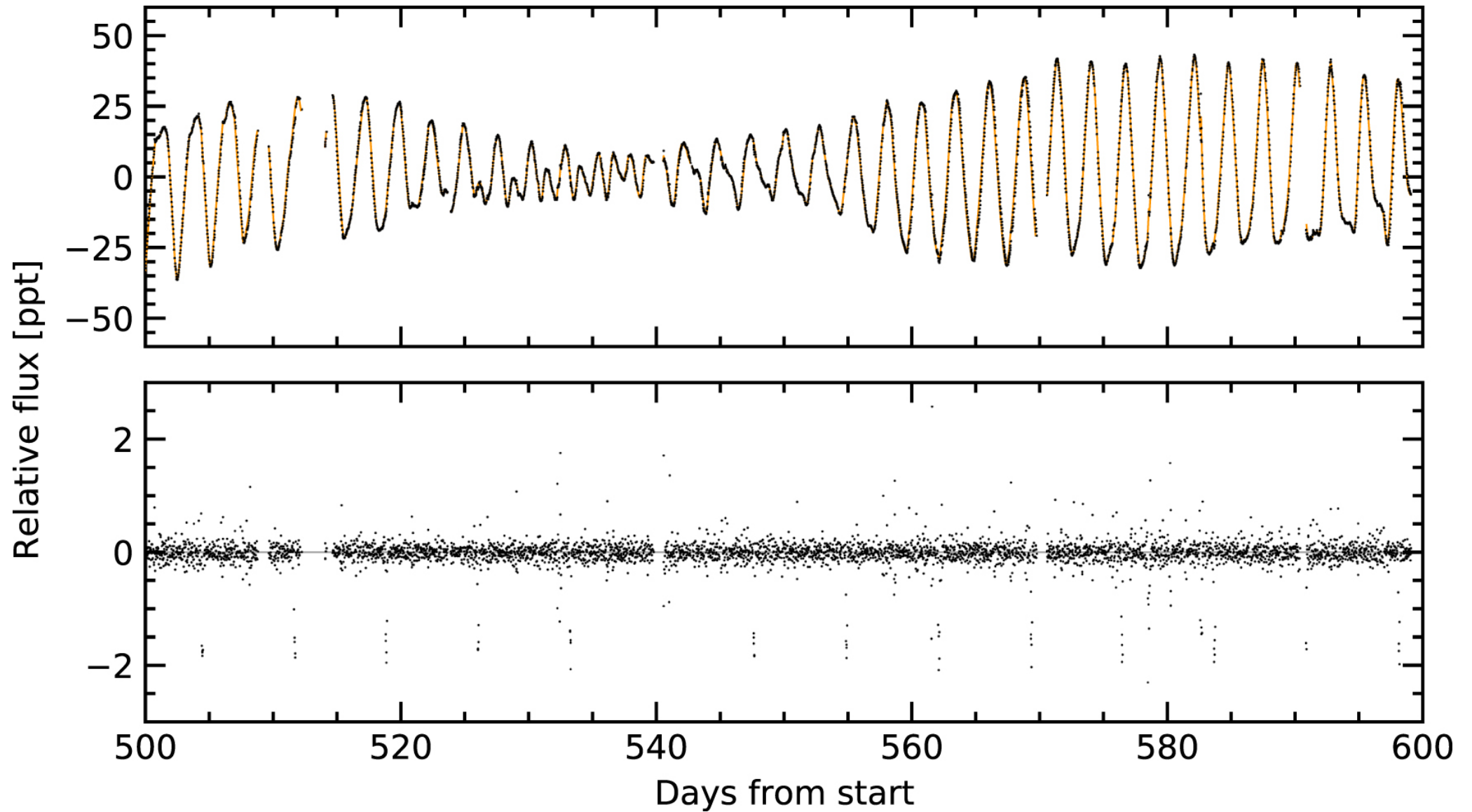
Figure 5. The light curve of Kepler 1627 from L. G. Bouma et al 2022 Astron. J. 163 doi:10.3847/1538-3881/ac4966 https://dx.doi.org/10.3847/1538-3881/ac4966 © 2022. The Author(s). Published by the American Astronomical Society.
