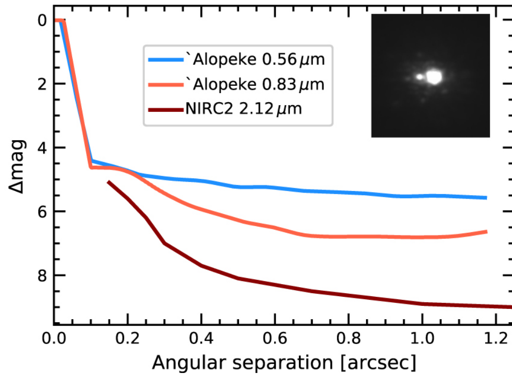
Figure 4. from L. G. Bouma et al 2022 Astron. J. 163 doi:10.3847/1538-3881/ac4966 https://dx.doi.org/10.3847/1538-3881/ac4966 © 2022. The Author(s). Published by the American Astronomical Society.
