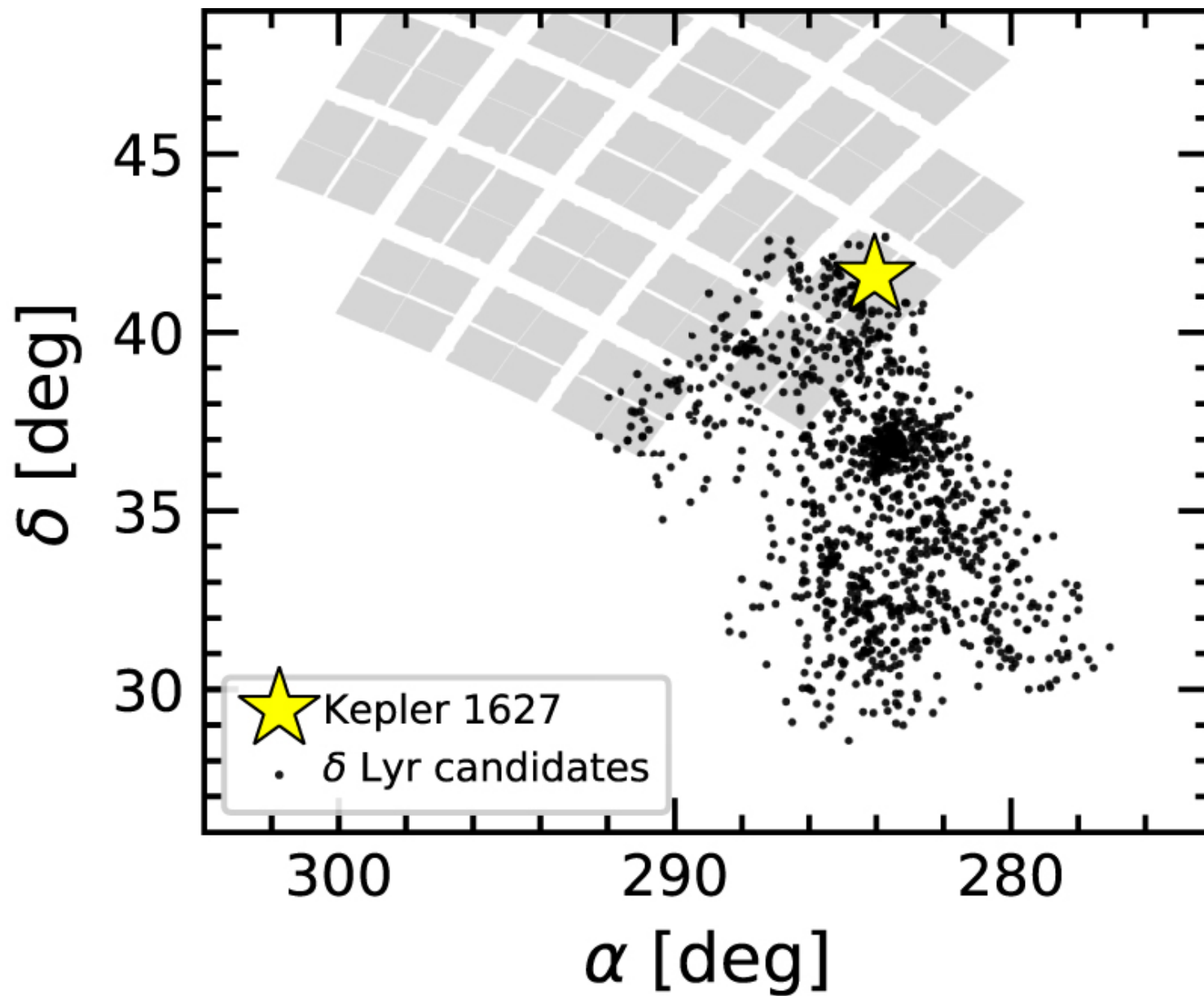
Figure 2. from L. G. Bouma et al 2022 Astron. J. 163 doi:10.3847/1538-3881/ac4966 https://dx.doi.org/10.3847/1538-3881/ac4966 © 2022. The Author(s). Published by the American Astronomical Society.
