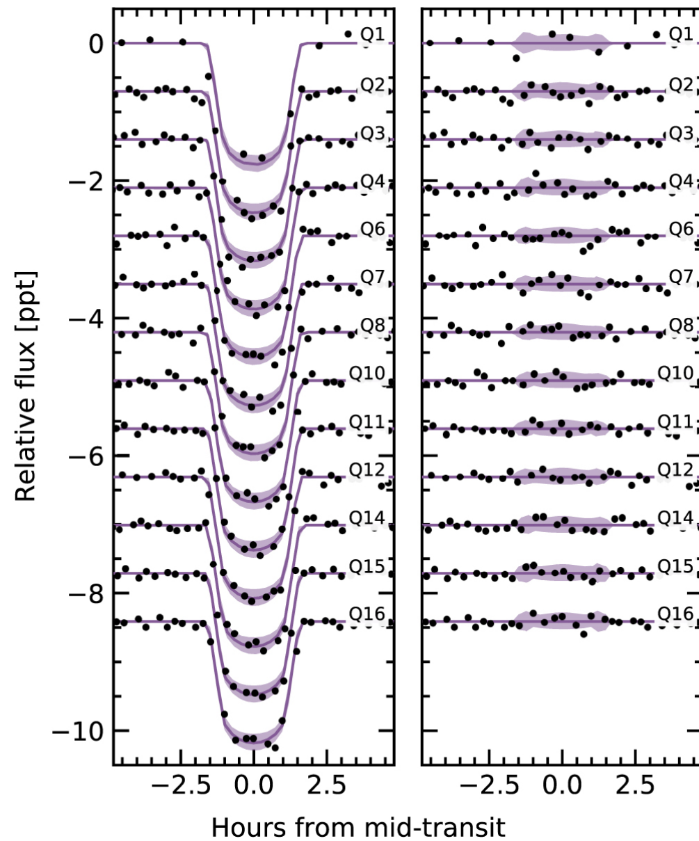
Figure 10. from L. G. Bouma et al 2022 Astron. J. 163 doi:10.3847/1538-3881/ac4966 https://dx.doi.org/10.3847/1538-3881/ac4966 © 2022. The Author(s). Published by the American Astronomical Society.
