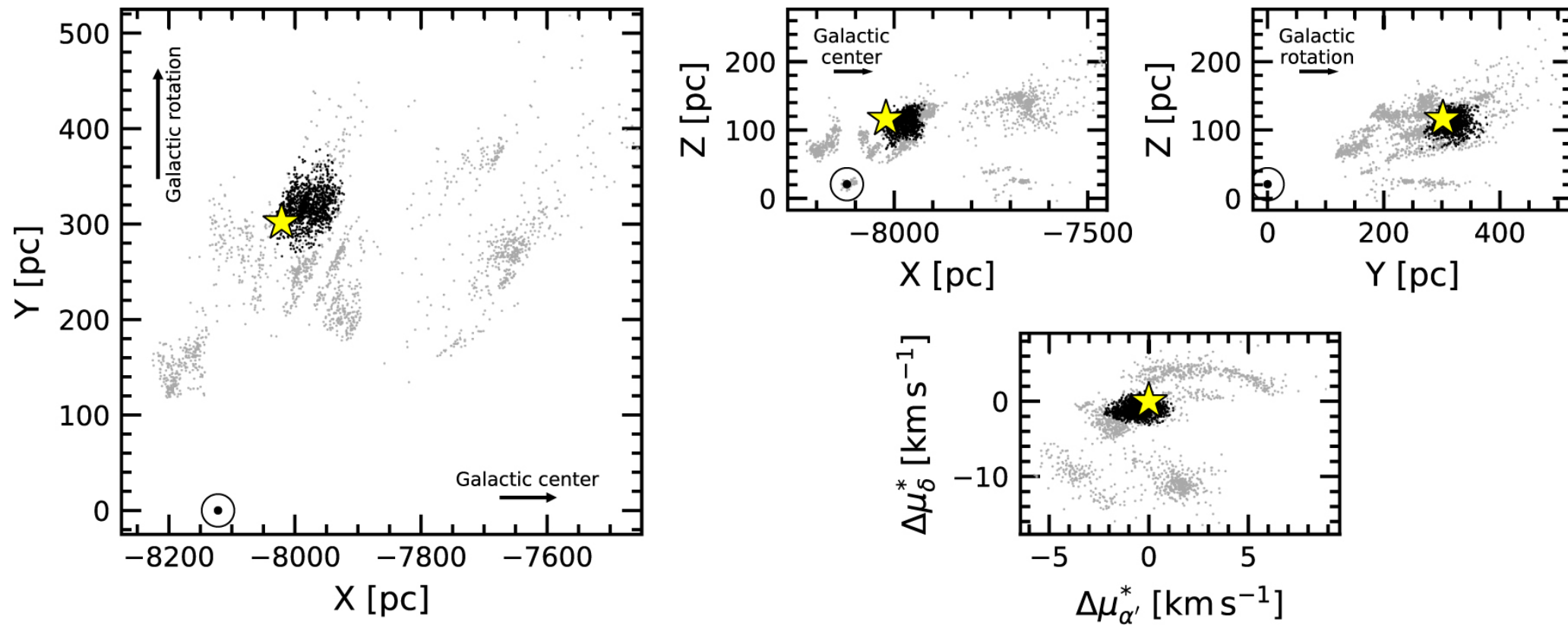
Figure 1. from L. G. Bouma et al 2022 Astron. J. 163 doi:10.3847/1538-3881/ac4966 https://dx.doi.org/10.3847/1538-3881/ac4966 © 2022. The Author(s). Published by the American Astronomical Society.
