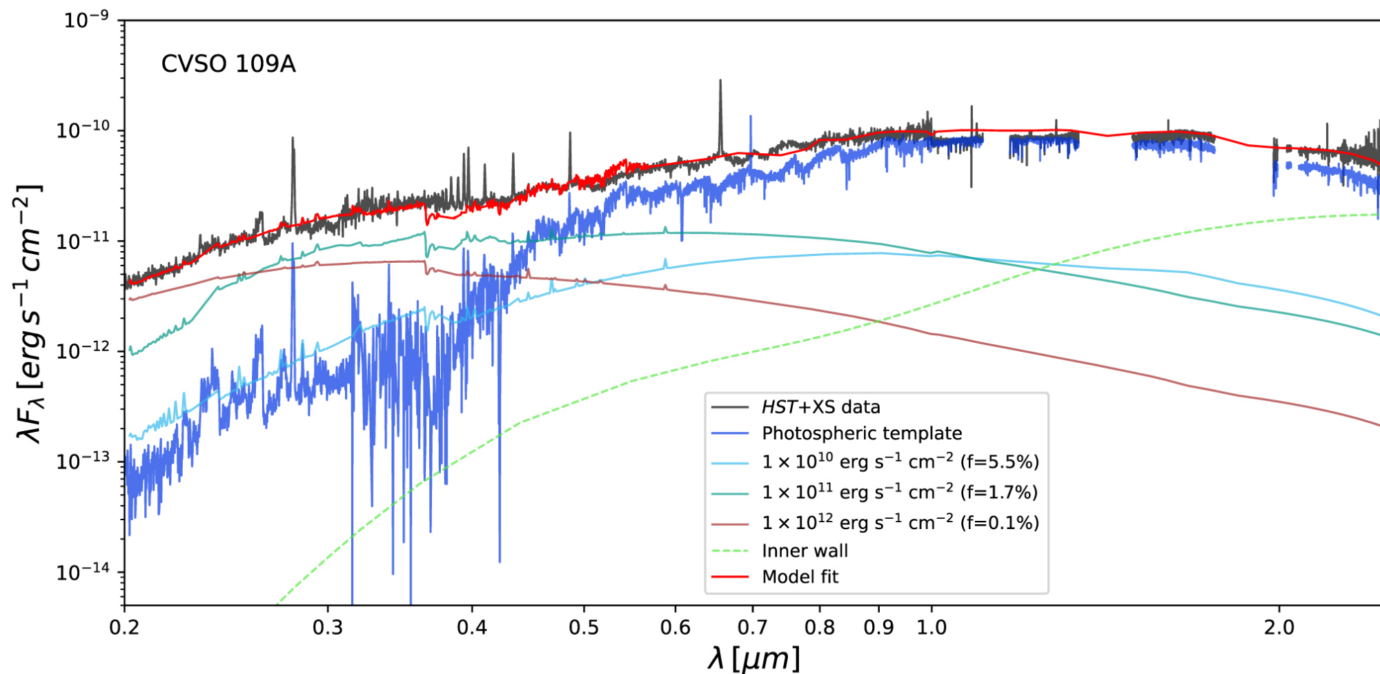
Figure 6. from The ODYSSEUS Survey. Motivation and First Results: Accretion, Ejection, and Disk Irradiation of CVSO 109 null 2022 AJ 163 114 doi:10.3847/1538-3881/ac479d https://dx.doi.org/10.3847/1538-3881/ac479d © 2022. The Author(s). Published by the American Astronomical Society.
