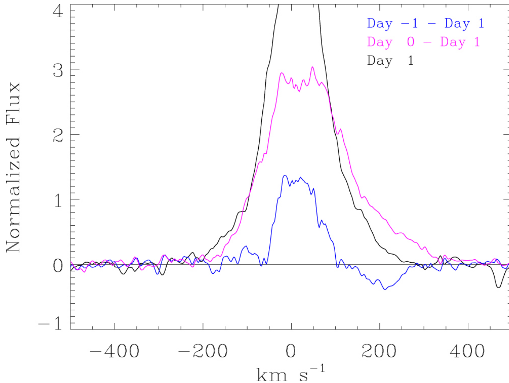
Figure 4. from The ODYSSEUS Survey. Motivation and First Results: Accretion, Ejection, and Disk Irradiation of CVSO 109 null 2022 AJ 163 114 doi:10.3847/1538-3881/ac479d https://dx.doi.org/10.3847/1538-3881/ac479d © 2022. The Author(s). Published by the American Astronomical Society.
