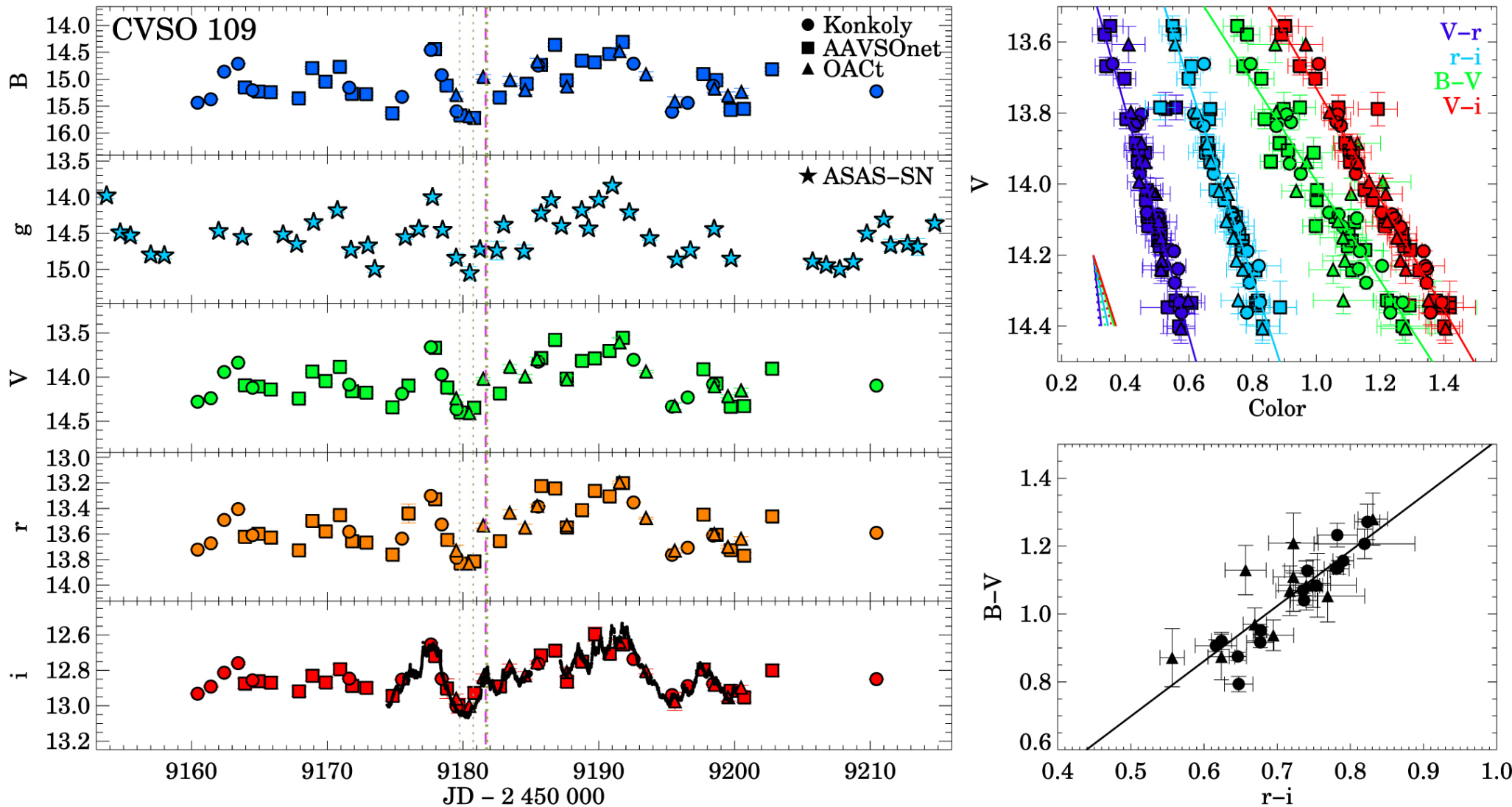
Figure 3. from The ODYSSEUS Survey. Motivation and First Results: Accretion, Ejection, and Disk Irradiation of CVSO 109 null 2022 AJ 163 114 doi:10.3847/1538-3881/ac479d https://dx.doi.org/10.3847/1538-3881/ac479d © 2022. The Author(s). Published by the American Astronomical Society.
