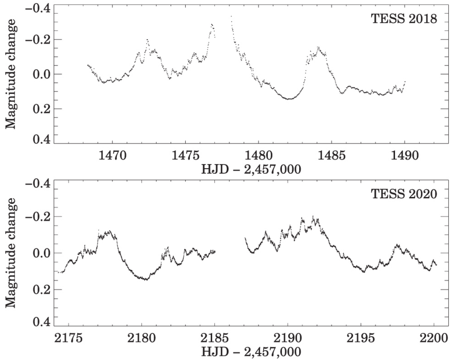
Figure 1. from The ODYSSEUS Survey. Motivation and First Results: Accretion, Ejection, and Disk Irradiation of CVSO 109 null 2022 AJ 163 114 doi:10.3847/1538-3881/ac479d https://dx.doi.org/10.3847/1538-3881/ac479d © 2022. The Author(s). Published by the American Astronomical Society.
