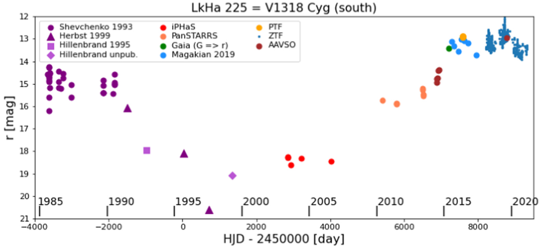
Figure 3. from LkH 225 (V1318 Cyg) South in Outburst null 2022 AJ 163 115 doi:10.3847/1538-3881/ac4752 https://dx.doi.org/10.3847/1538-3881/ac4752
