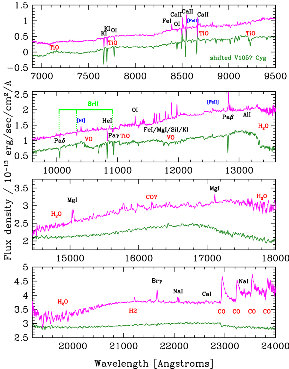
Figure 10. from LkH 225 (V1318 Cyg) South in Outburst null 2022 AJ 163 115 doi:10.3847/1538-3881/ac4752 https://dx.doi.org/10.3847/1538-3881/ac4752
