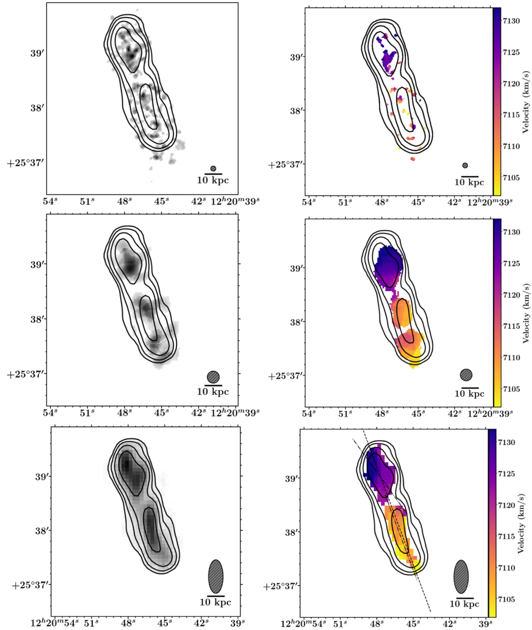
Figure 2. from Lukas Leisman et al 2021 Astron. J. 162 doi:10.3847/1538-3881/ac2a38 https://dx.doi.org/10.3847/1538-3881/ac2a38 © 2021. The American Astronomical Society. All rights reserved.
