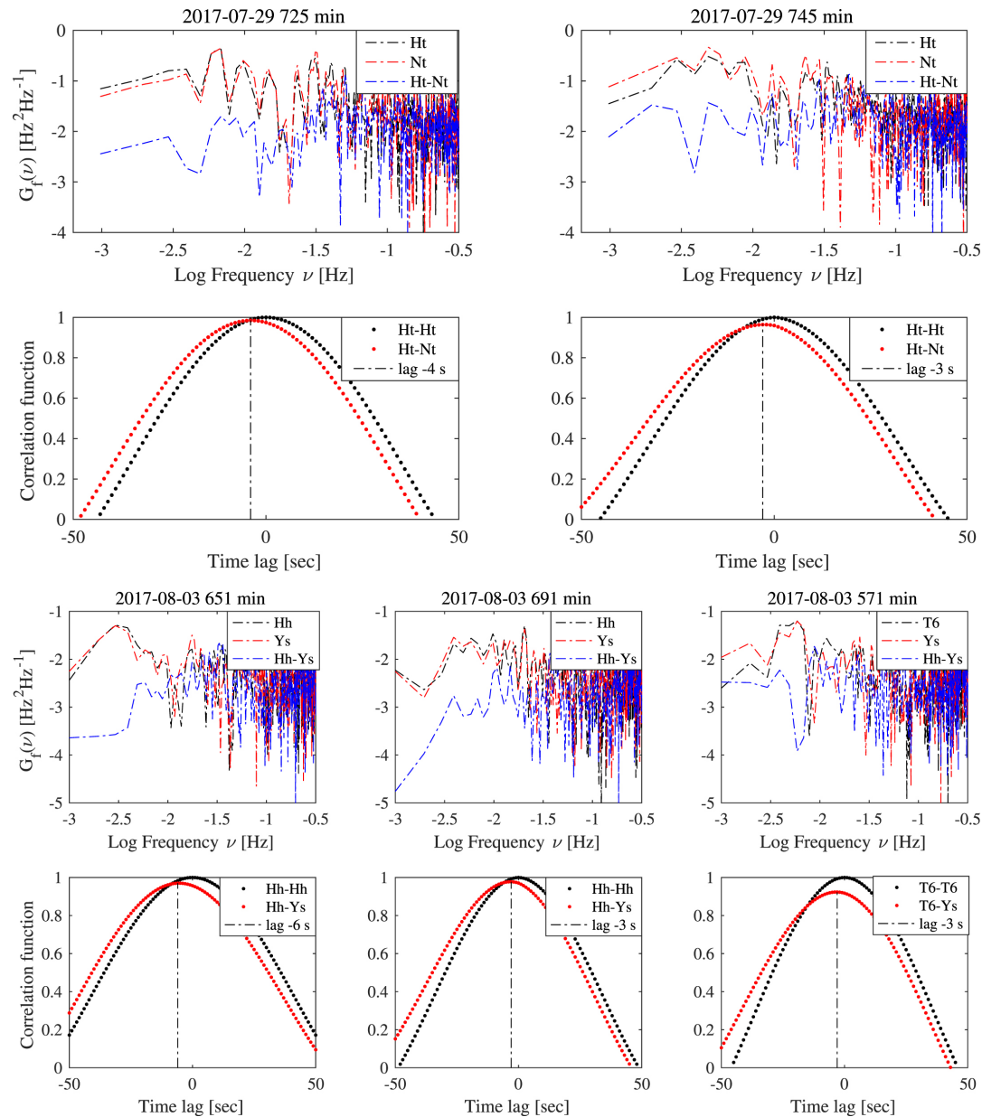
Figure 9. from VLBI Data Processing on Coronal Radio-sounding Experiments of Mars Express null 2021 AJ 162 141 doi:10.3847/1538-3881/ac0dc1 https://dx.doi.org/10.3847/1538-3881/ac0dc1
