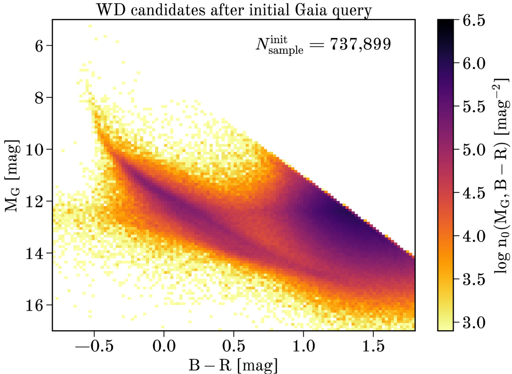
Figure 2. from Selection Functions in Astronomical Data Modeling, with the Space Density of White Dwarfs as a Worked Example null 2021 AJ 162 142 doi:10.3847/1538-3881/ac0c13 https://dx.doi.org/10.3847/1538-3881/ac0c13 © 2021. The Author(s). Published by the American Astronomical Society.
