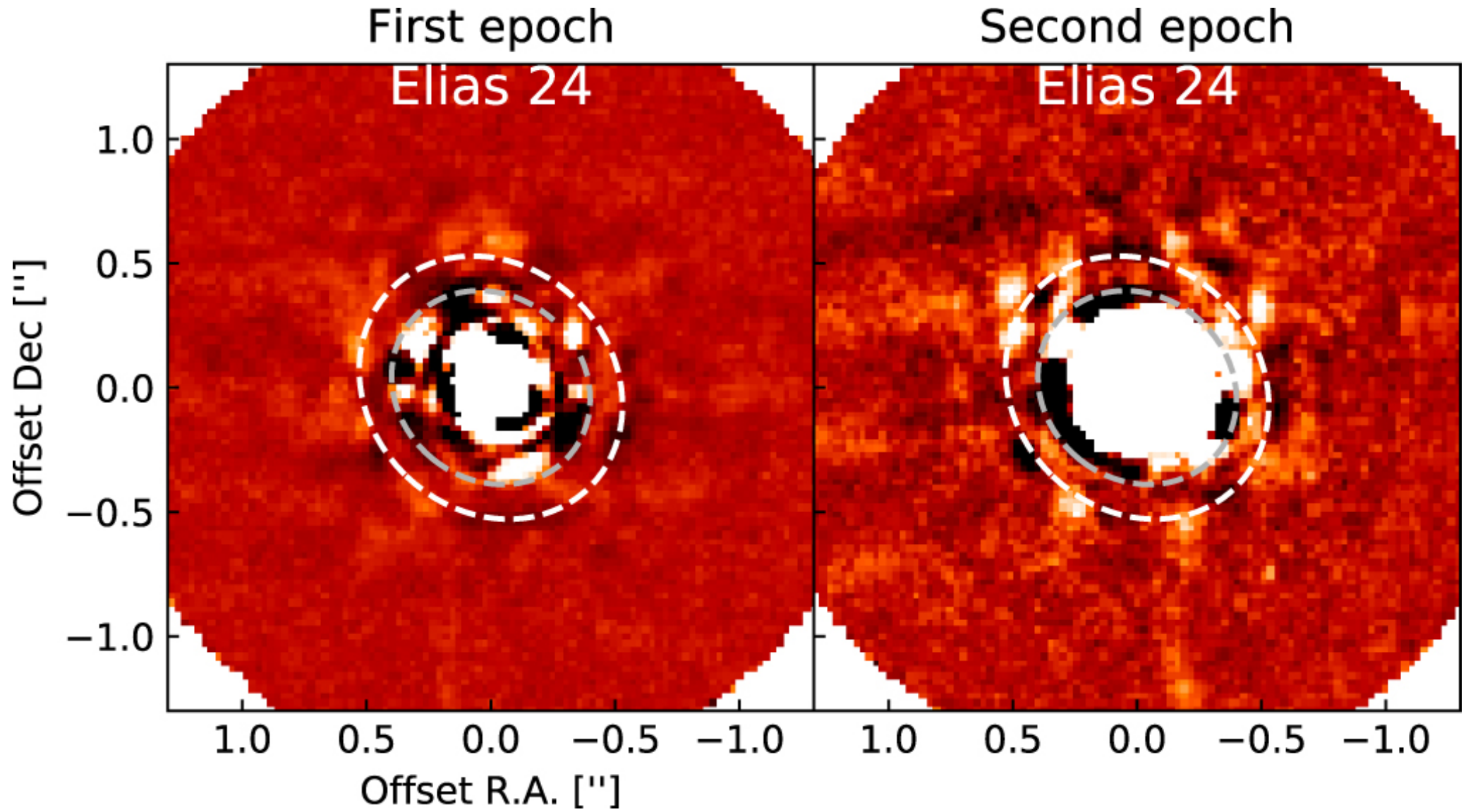
Figure 9. from A Search for Companions via Direct Imaging in the DSHARP Planet-forming Disks null 2021 AJ 161 146 doi:10.3847/1538-3881/abd40d https://dx.doi.org/10.3847/1538-3881/abd40d © 2021. The American Astronomical Society. All rights reserved.
