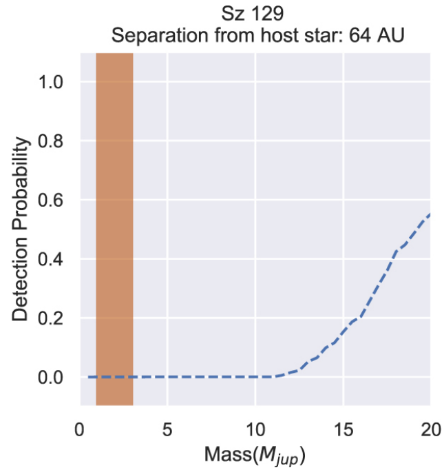
Figure 8. from A Search for Companions via Direct Imaging in the DSHARP Planet-forming Disks null 2021 AJ 161 146 doi:10.3847/1538-3881/abd40d https://dx.doi.org/10.3847/1538-3881/abd40d © 2021. The American Astronomical Society. All rights reserved.
