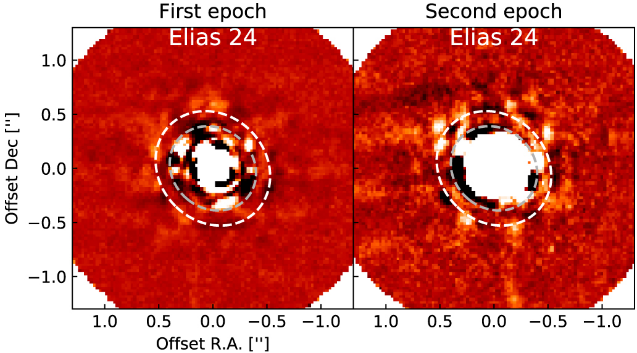
Figure 6. from A Search for Companions via Direct Imaging in the DSHARP Planet-forming Disks null 2021 AJ 161 146 doi:10.3847/1538-3881/abd40d https://dx.doi.org/10.3847/1538-3881/abd40d © 2021. The American Astronomical Society. All rights reserved.
