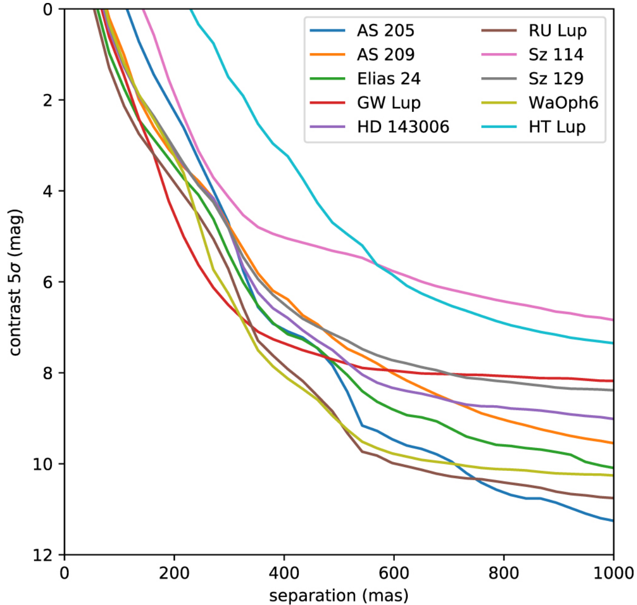
Figure 2. from A Search for Companions via Direct Imaging in the DSHARP Planet-forming Disks null 2021 AJ 161 146 doi:10.3847/1538-3881/abd40d https://dx.doi.org/10.3847/1538-3881/abd40d © 2021. The American Astronomical Society. All rights reserved.
