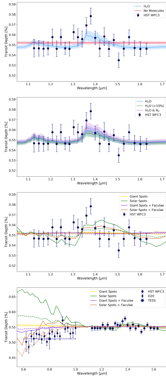
Figure 8. from Hubble WFC3 Spectroscopy of the Habitable-zone Super-Earth LHS 1140 b null 2021 AJ 161 44 doi:10.3847/1538-3881/abc6a5 https://dx.doi.org/10.3847/1538-3881/abc6a5 © 2020. The American Astronomical Society. All rights reserved.
