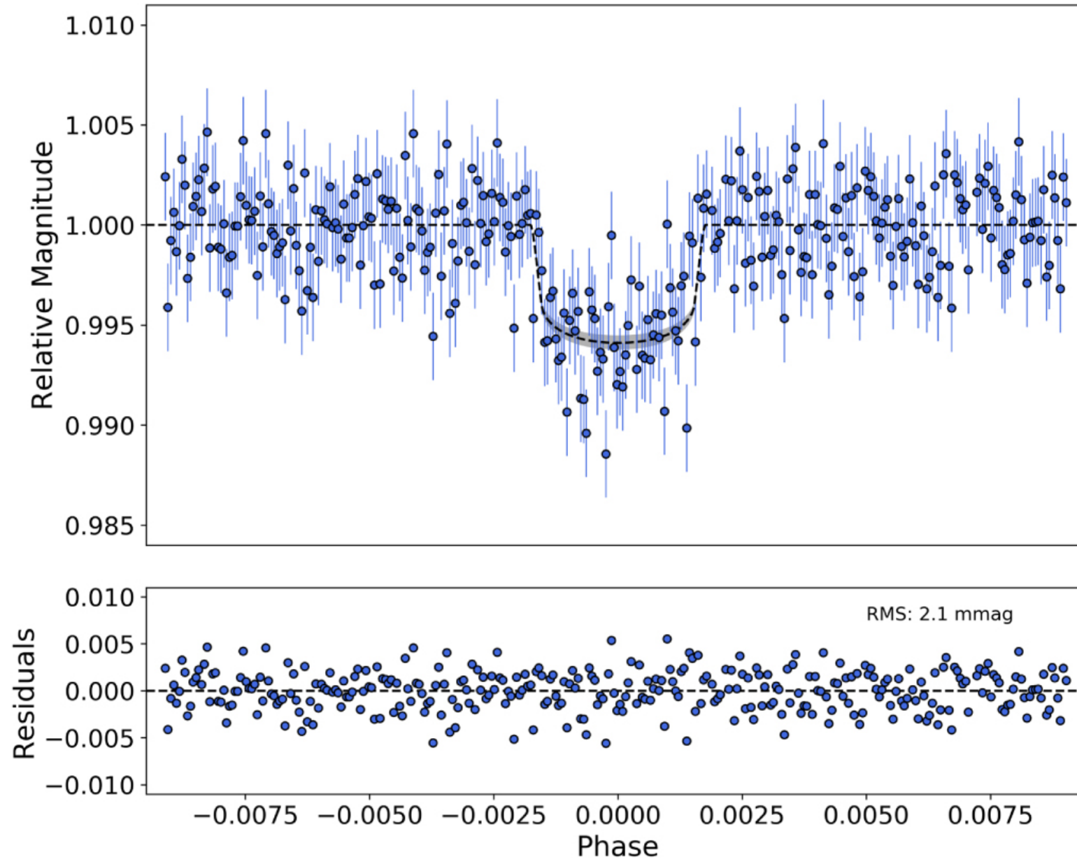
Figure 7. from Hubble WFC3 Spectroscopy of the Habitable-zone Super-Earth LHS 1140 b null 2021 AJ 161 44 doi:10.3847/1538-3881/abc6a5 https://dx.doi.org/10.3847/1538-3881/abc6a5 © 2020. The American Astronomical Society. All rights reserved.
