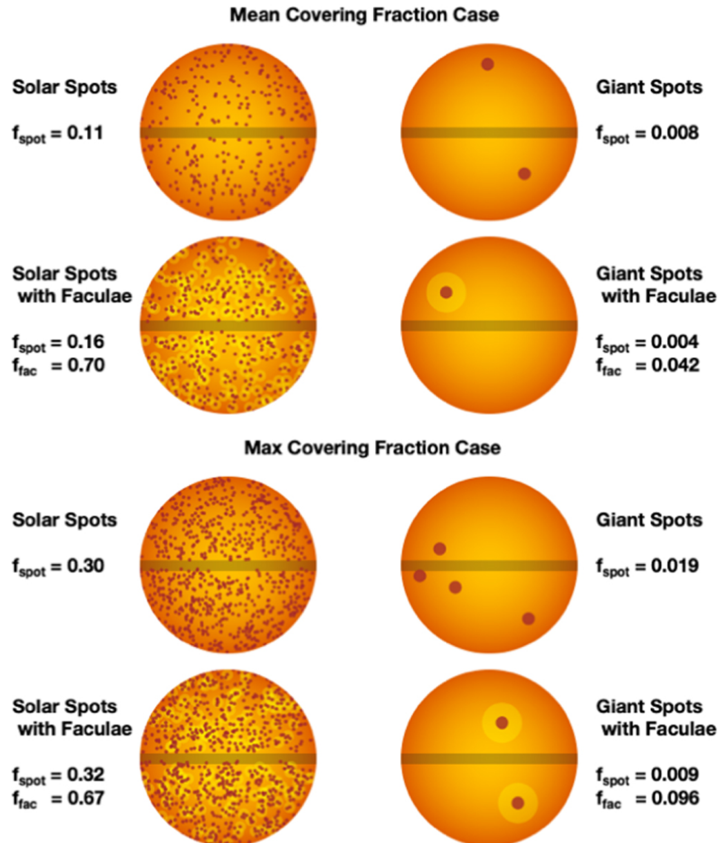
Figure 6. from Hubble WFC3 Spectroscopy of the Habitable-zone Super-Earth LHS 1140 b null 2021 AJ 161 44 doi:10.3847/1538-3881/abc6a5 https://dx.doi.org/10.3847/1538-3881/abc6a5 © 2020. The American Astronomical Society. All rights reserved.
