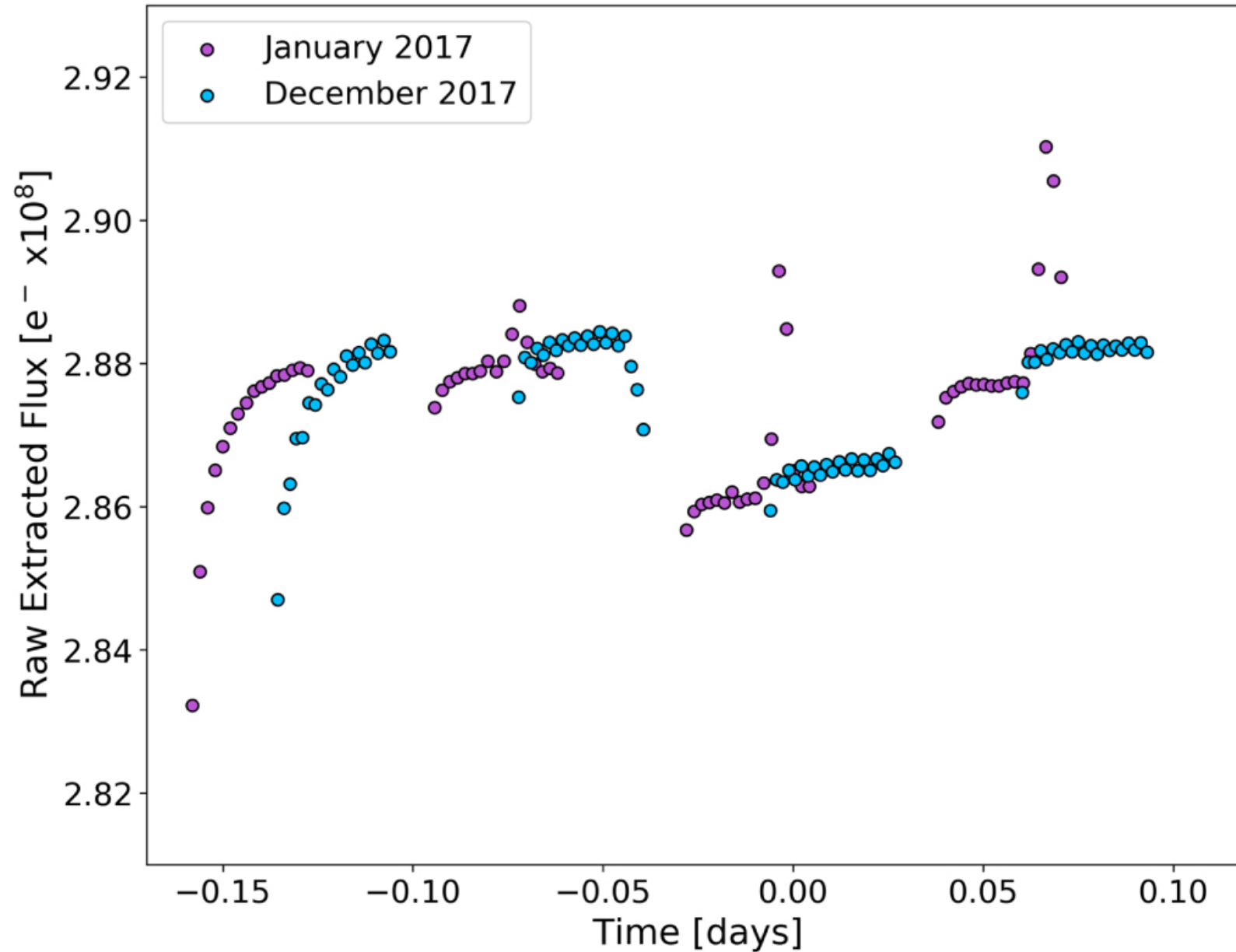
Figure 2. from Hubble WFC3 Spectroscopy of the Habitable-zone Super-Earth LHS 1140 b null 2021 AJ 161 44 doi:10.3847/1538-3881/abc6a5 https://dx.doi.org/10.3847/1538-3881/abc6a5 © 2020. The American Astronomical Society. All rights reserved.
