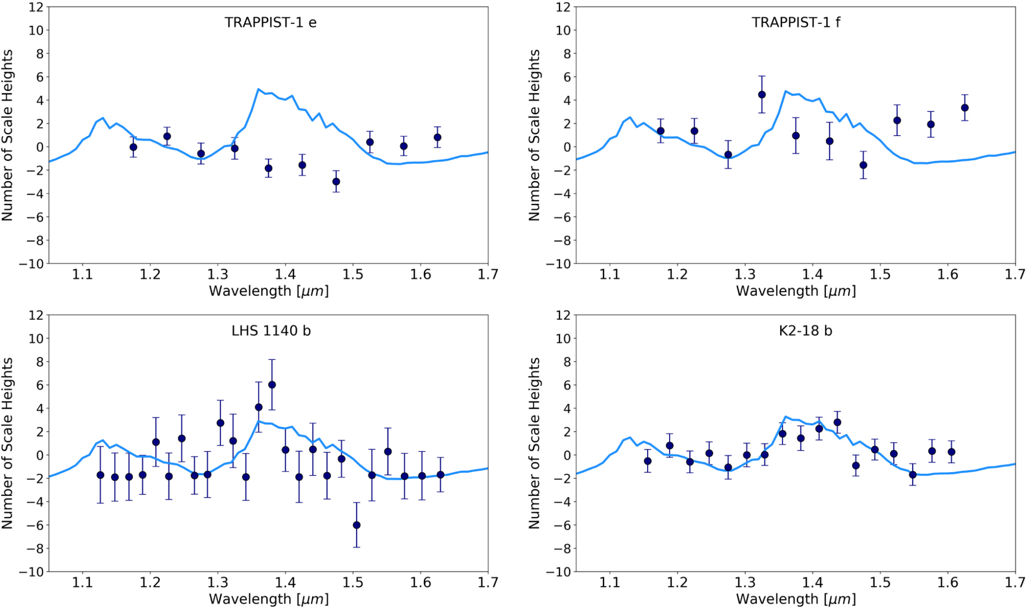
Figure 18. from Hubble WFC3 Spectroscopy of the Habitable-zone Super-Earth LHS 1140 b null 2021 AJ 161 44 doi:10.3847/1538-3881/abc6a5 https://dx.doi.org/10.3847/1538-3881/abc6a5 © 2020. The American Astronomical Society. All rights reserved.
