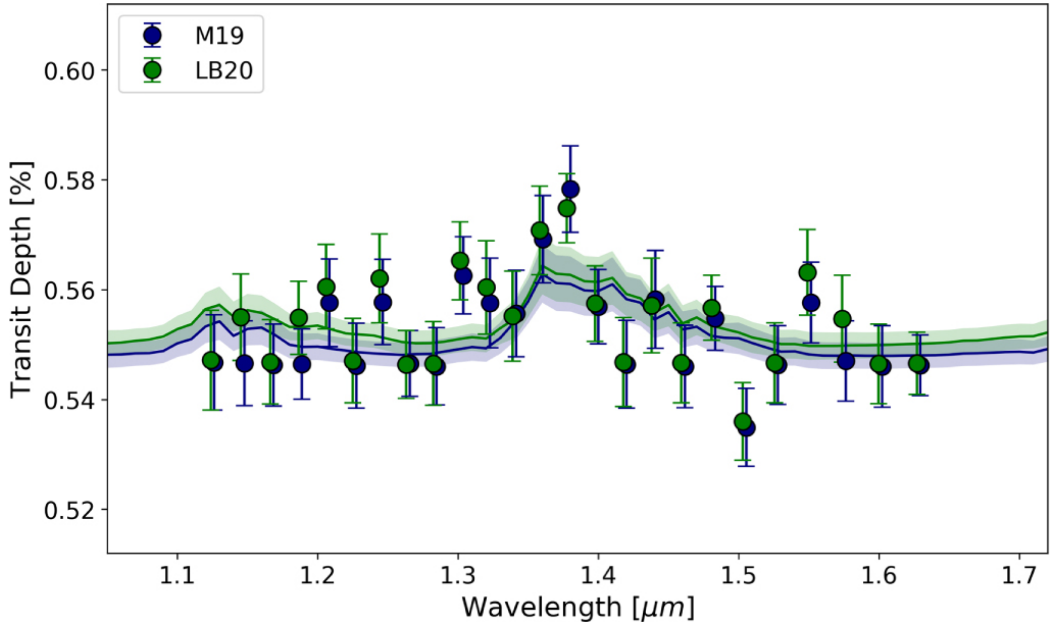
Figure 17. from Hubble WFC3 Spectroscopy of the Habitable-zone Super-Earth LHS 1140 b null 2021 AJ 161 44 doi:10.3847/1538-3881/abc6a5 https://dx.doi.org/10.3847/1538-3881/abc6a5 © 2020. The American Astronomical Society. All rights reserved.
