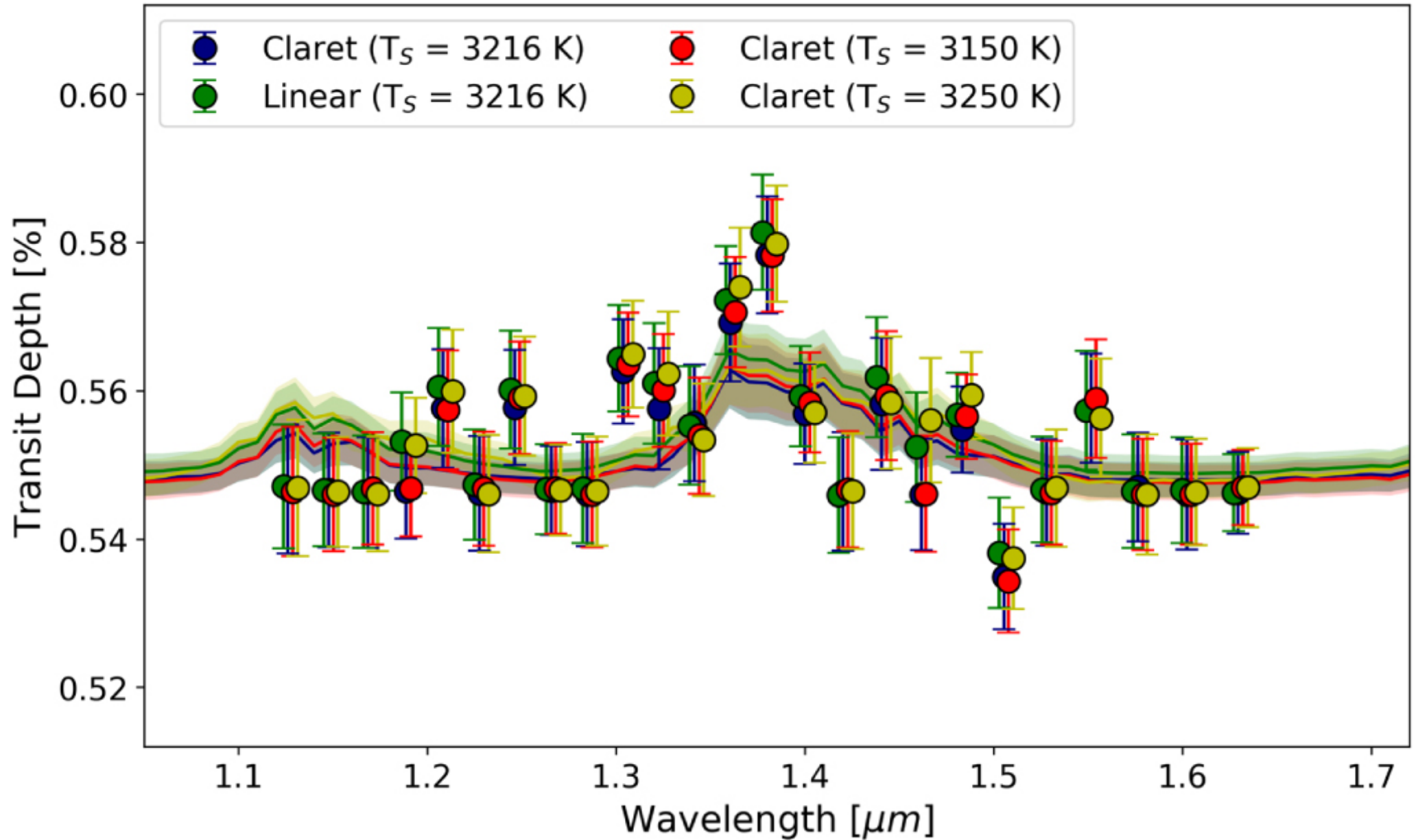
Figure 16. from Hubble WFC3 Spectroscopy of the Habitable-zone Super-Earth LHS 1140 b null 2021 AJ 161 44 doi:10.3847/1538-3881/abc6a5 https://dx.doi.org/10.3847/1538-3881/abc6a5 © 2020. The American Astronomical Society. All rights reserved.
