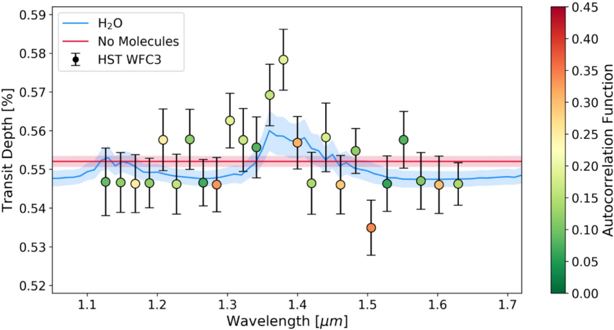
Figure 15. from Hubble WFC3 Spectroscopy of the Habitable-zone Super-Earth LHS 1140 b null 2021 AJ 161 44 doi:10.3847/1538-3881/abc6a5 https://dx.doi.org/10.3847/1538-3881/abc6a5 © 2020. The American Astronomical Society. All rights reserved.
