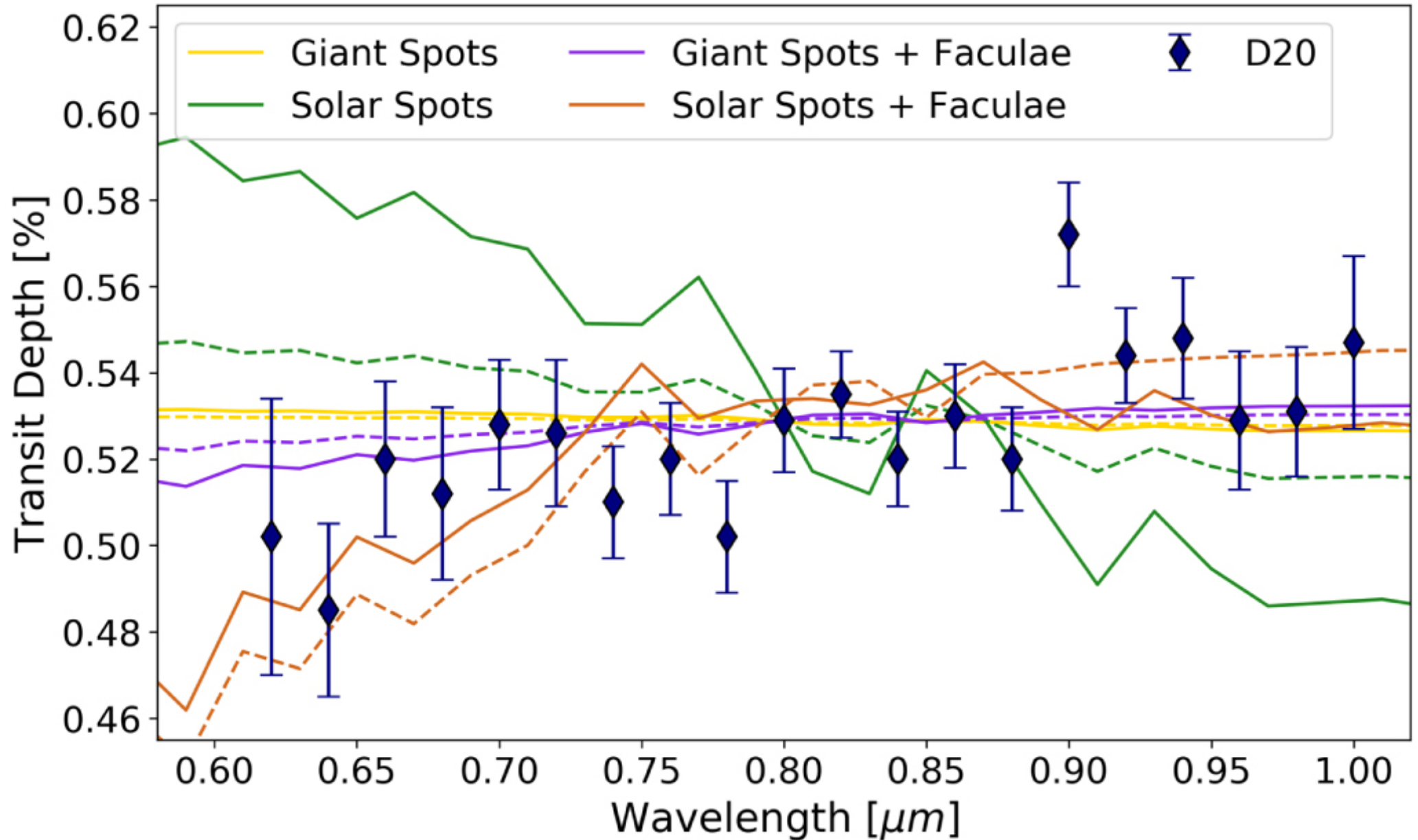
Figure 12. from Hubble WFC3 Spectroscopy of the Habitable-zone Super-Earth LHS 1140 b null 2021 AJ 161 44 doi:10.3847/1538-3881/abc6a5 https://dx.doi.org/10.3847/1538-3881/abc6a5 © 2020. The American Astronomical Society. All rights reserved.
