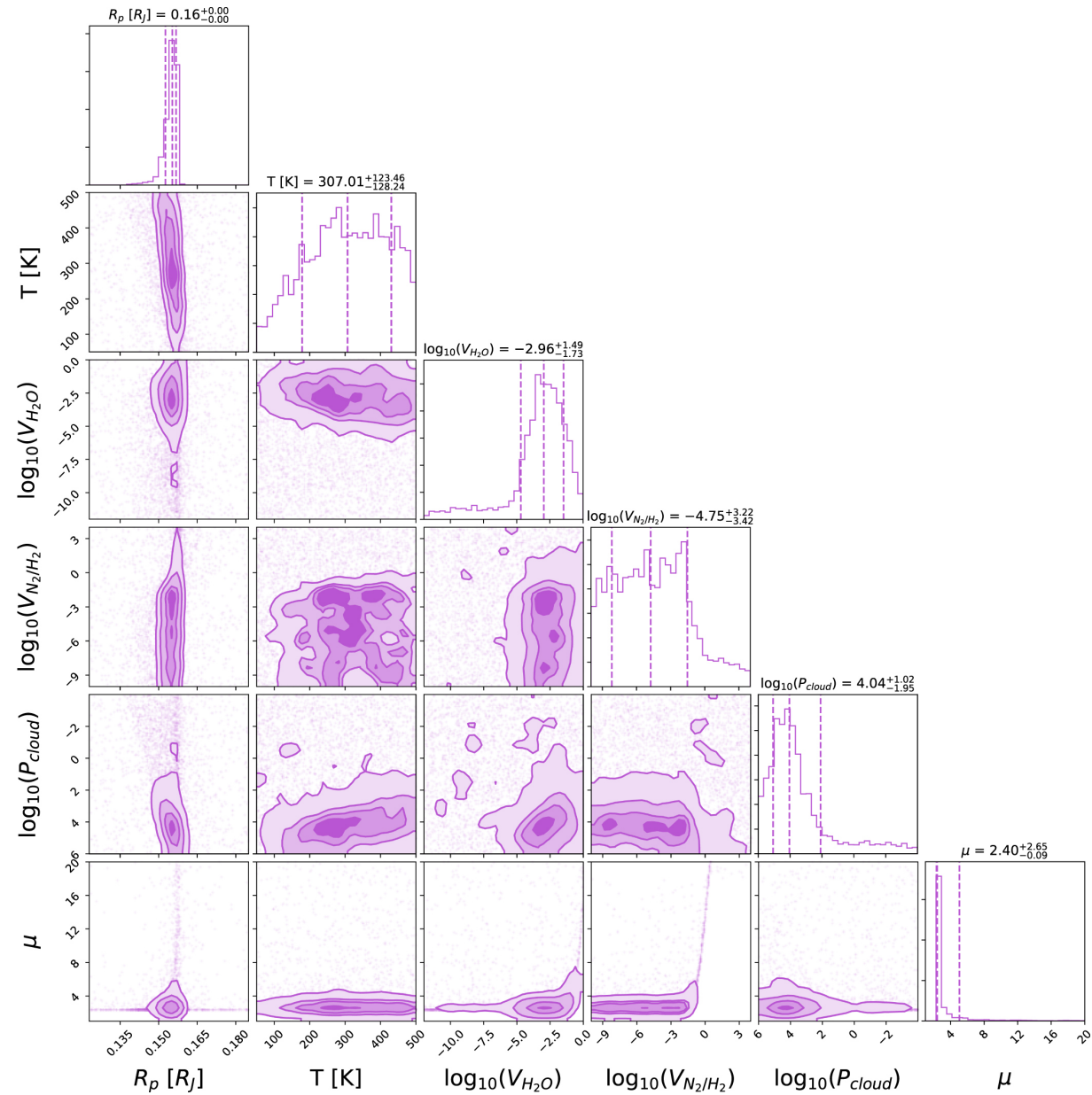
Figure 11. from Hubble WFC3 Spectroscopy of the Habitable-zone Super-Earth LHS 1140 b null 2021 AJ 161 44 doi:10.3847/1538-3881/abc6a5 https://dx.doi.org/10.3847/1538-3881/abc6a5 © 2020. The American Astronomical Society. All rights reserved.
