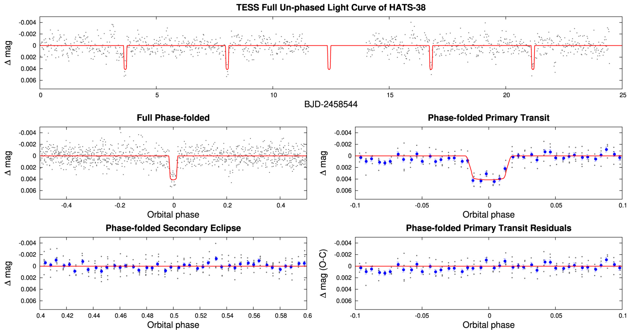
Figure 3. from HATS-37Ab and HATS-38b: Two Transiting Hot Neptunes in the Desert null 2020 AJ 160 222 doi:10.3847/1538-3881/aba530 https://dx.doi.org/10.3847/1538-3881/aba530 © 2020. The American Astronomical Society. All rights reserved.
