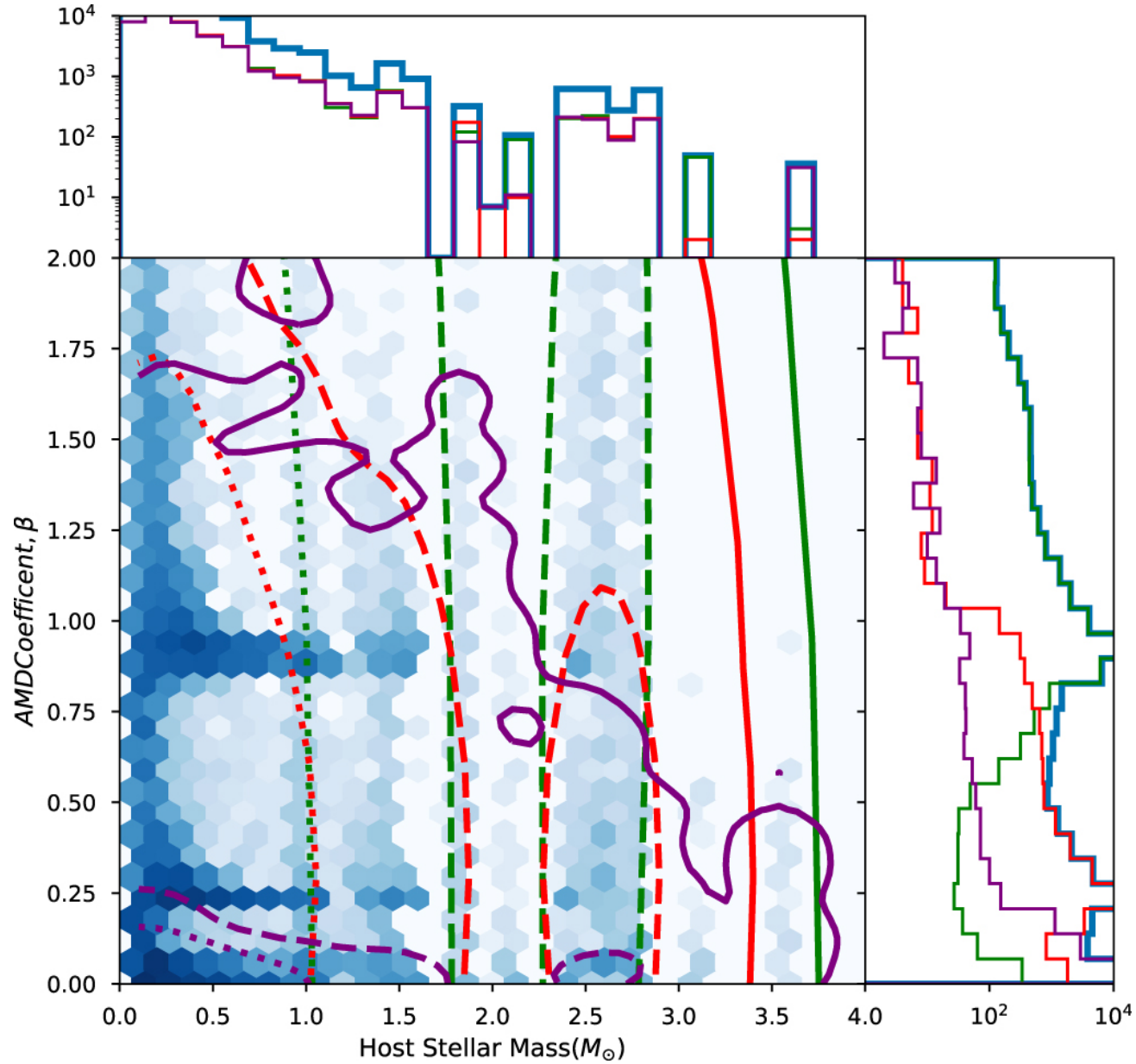
Figure 9. from TYCHO: Realistically Simulating Exoplanets within Stellar Clusters. I. Improving the Monte Carlo Approach null 2020 AJ 160 126 doi:10.3847/1538-3881/aba2ea https://dx.doi.org/10.3847/1538-3881/aba2ea © 2020. The American Astronomical Society. All rights reserved.
