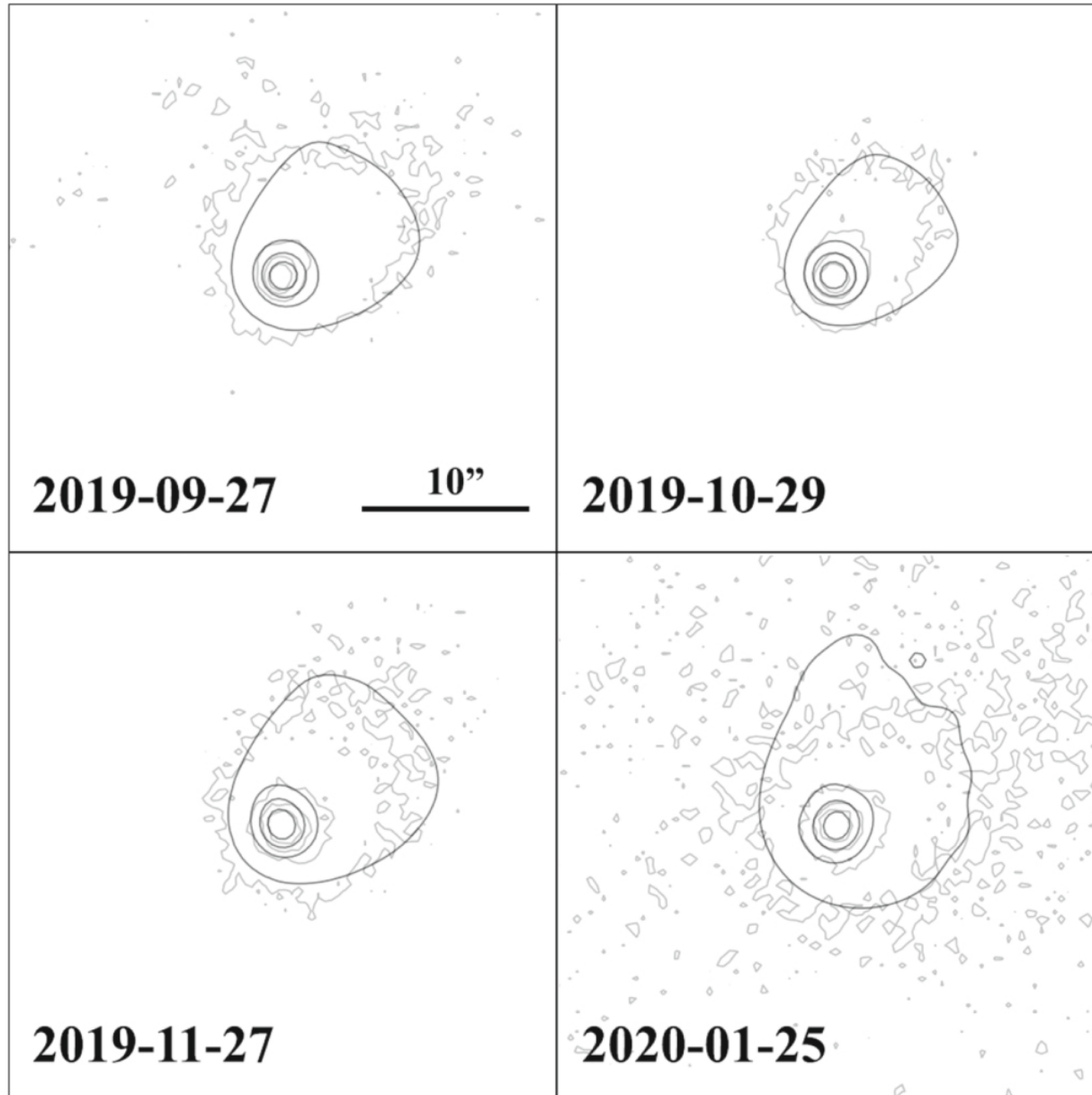
Figure 8. from Physical Characterization of Interstellar Comet 2I/2019 Q4 (Borisov) null 2020 AJ 160 92 doi:10.3847/1538-3881/ab9df8 https://dx.doi.org/10.3847/1538-3881/ab9df8 © 2020. The American Astronomical Society. All rights reserved.
