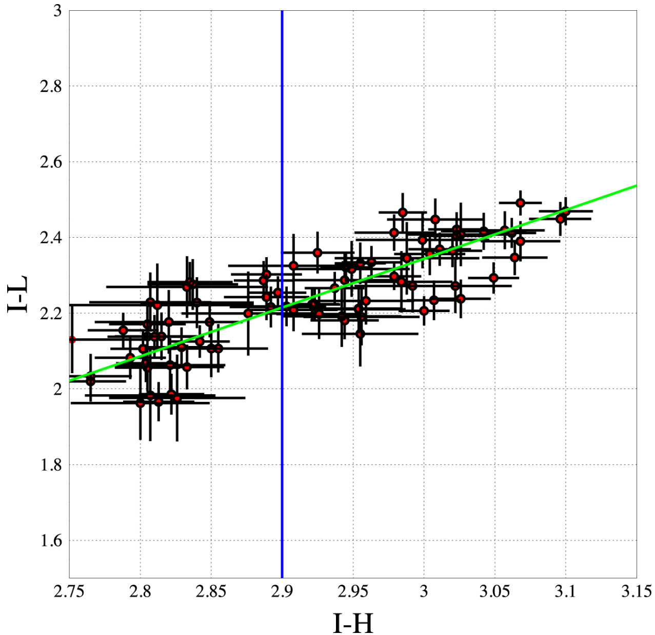
Figure 7. from OGLE-2017-BLG-0406: Spitzer Microlens Parallax Reveals Saturn-mass Planet Orbiting M-dwarf Host in the Inner Galactic Disk null 2020 AJ 160 74 doi:10.3847/1538-3881/ab9ac3 https://dx.doi.org/10.3847/1538-3881/ab9ac3 © 2020. The American Astronomical Society. All rights reserved.
