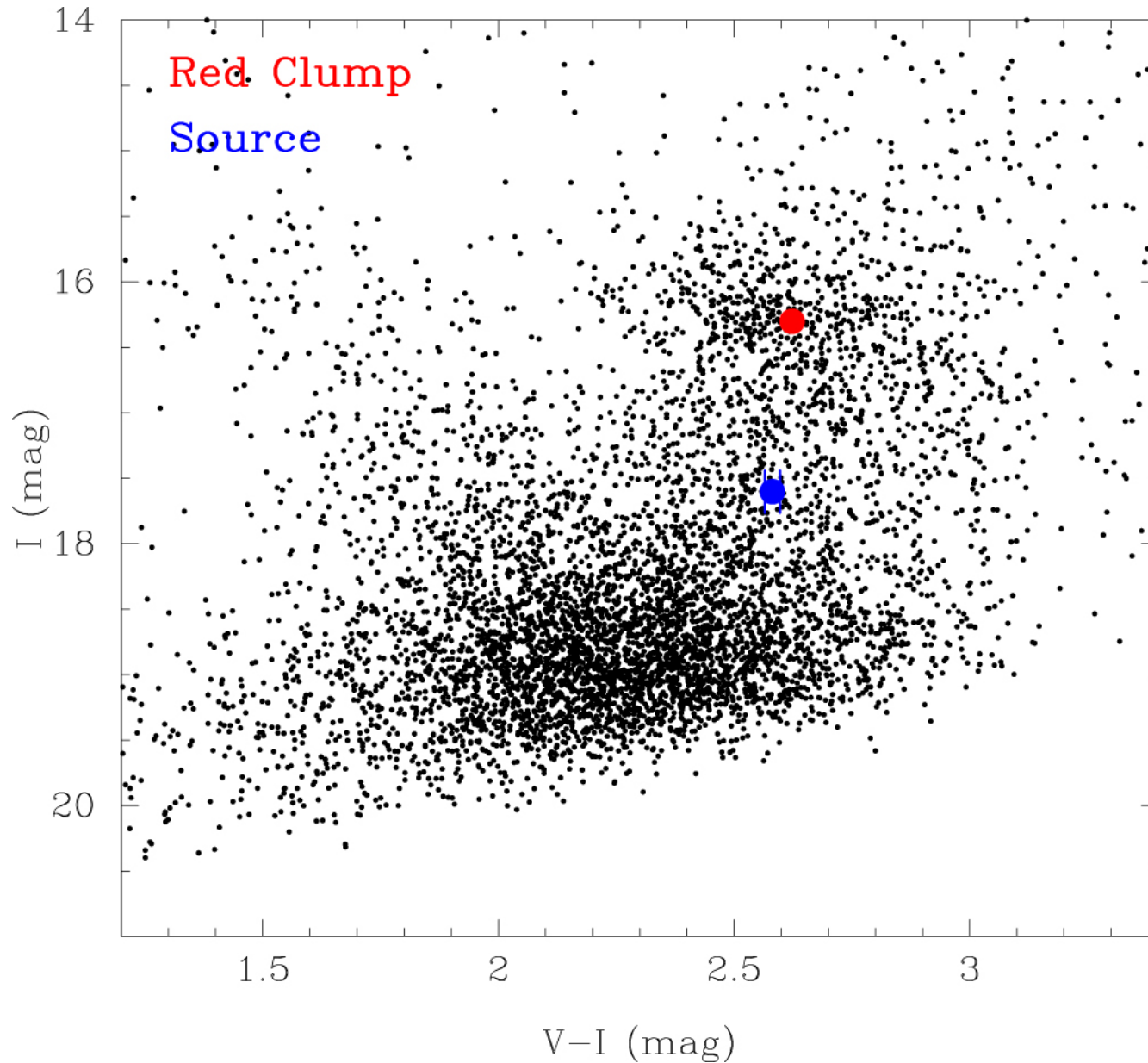
Figure 4. from OGLE-2017-BLG-0406: Spitzer Microlens Parallax Reveals Saturn-mass Planet Orbiting M-dwarf Host in the Inner Galactic Disk null 2020 AJ 160 74 doi:10.3847/1538-3881/ab9ac3 https://dx.doi.org/10.3847/1538-3881/ab9ac3 © 2020. The American Astronomical Society. All rights reserved.
