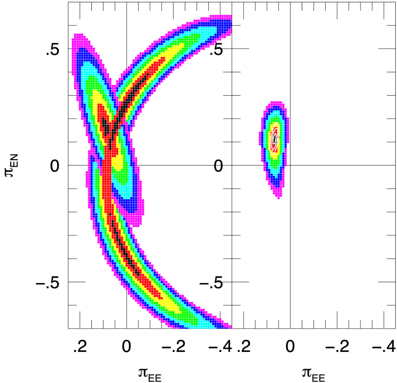
Figure 3. from OGLE-2017-BLG-0406: Spitzer Microlens Parallax Reveals Saturn-mass Planet Orbiting M-dwarf Host in the Inner Galactic Disk null 2020 AJ 160 74 doi:10.3847/1538-3881/ab9ac3 https://dx.doi.org/10.3847/1538-3881/ab9ac3 © 2020. The American Astronomical Society. All rights reserved.
