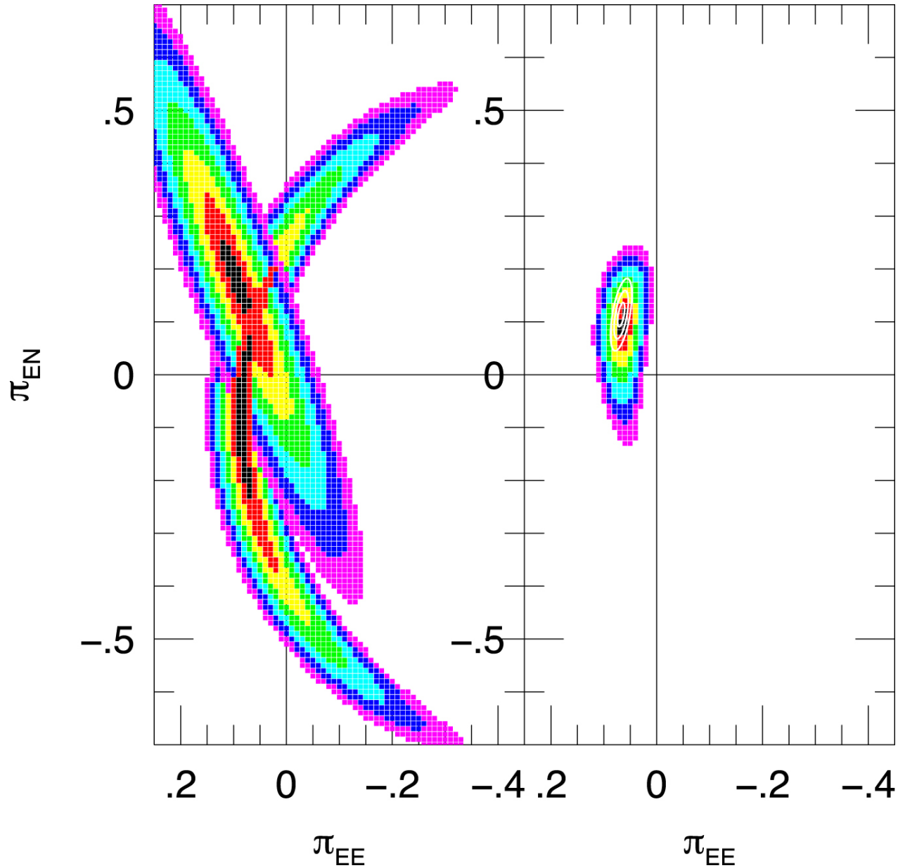
Figure A1. from OGLE-2017-BLG-0406: Spitzer Microlens Parallax Reveals Saturn-mass Planet Orbiting M-dwarf Host in the Inner Galactic Disk null 2020 AJ 160 74 doi:10.3847/1538-3881/ab9ac3 https://dx.doi.org/10.3847/1538-3881/ab9ac3 © 2020. The American Astronomical Society. All rights reserved.
