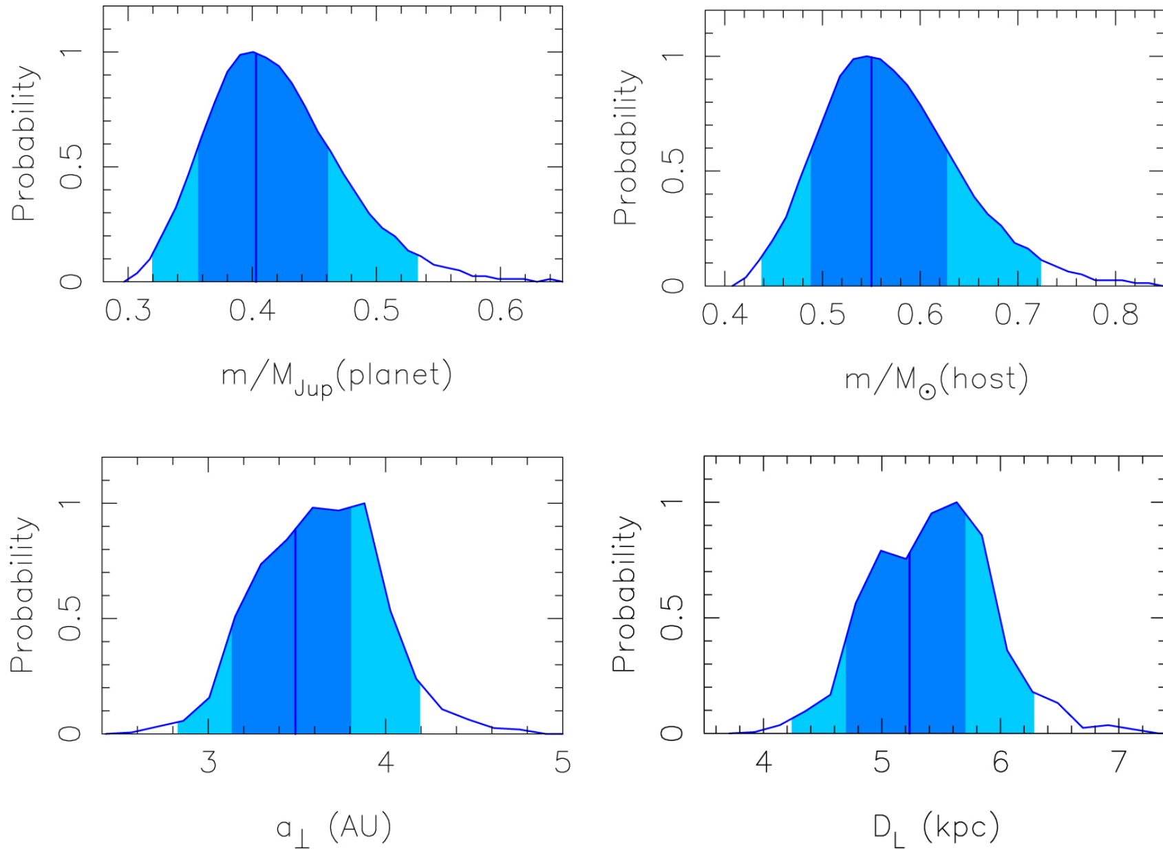
Figure 10. from OGLE-2017-BLG-0406: Spitzer Microlens Parallax Reveals Saturn-mass Planet Orbiting M-dwarf Host in the Inner Galactic Disk null 2020 AJ 160 74 doi:10.3847/1538-3881/ab9ac3 https://dx.doi.org/10.3847/1538-3881/ab9ac3 © 2020. The American Astronomical Society. All rights reserved.
