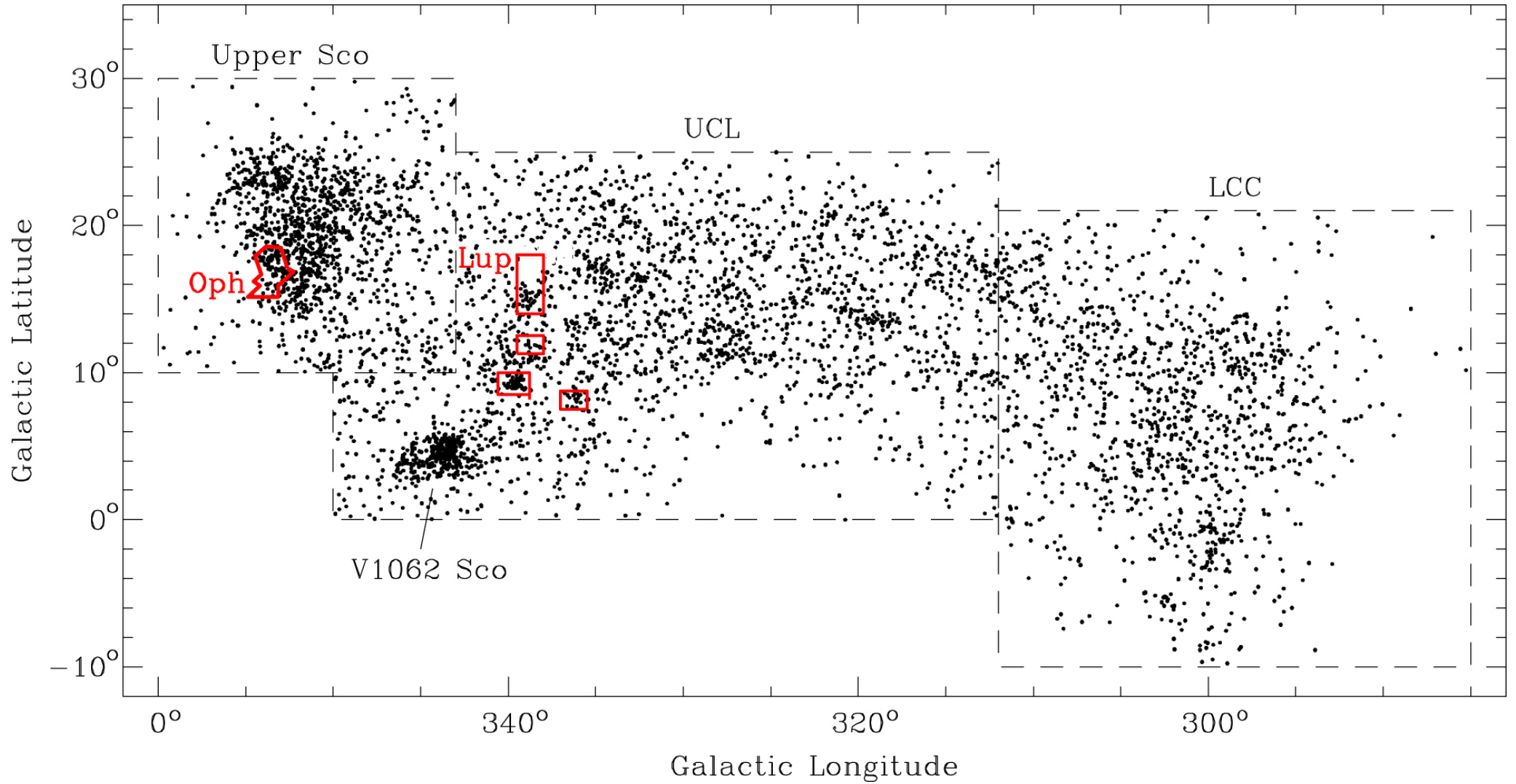
Figure 5. from Refining the Census of the Upper Scorpius Association with Gaia null 2020 AJ 160 44 doi:10.3847/1538-3881/ab9599 https://dx.doi.org/10.3847/1538-3881/ab9599 © 2020. The American Astronomical Society. All rights reserved.
