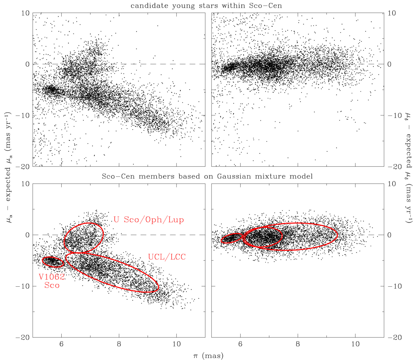
Figure 4. from Refining the Census of the Upper Scorpius Association with Gaia null 2020 AJ 160 44 doi:10.3847/1538-3881/ab9599 https://dx.doi.org/10.3847/1538-3881/ab9599 © 2020. The American Astronomical Society. All rights reserved.
