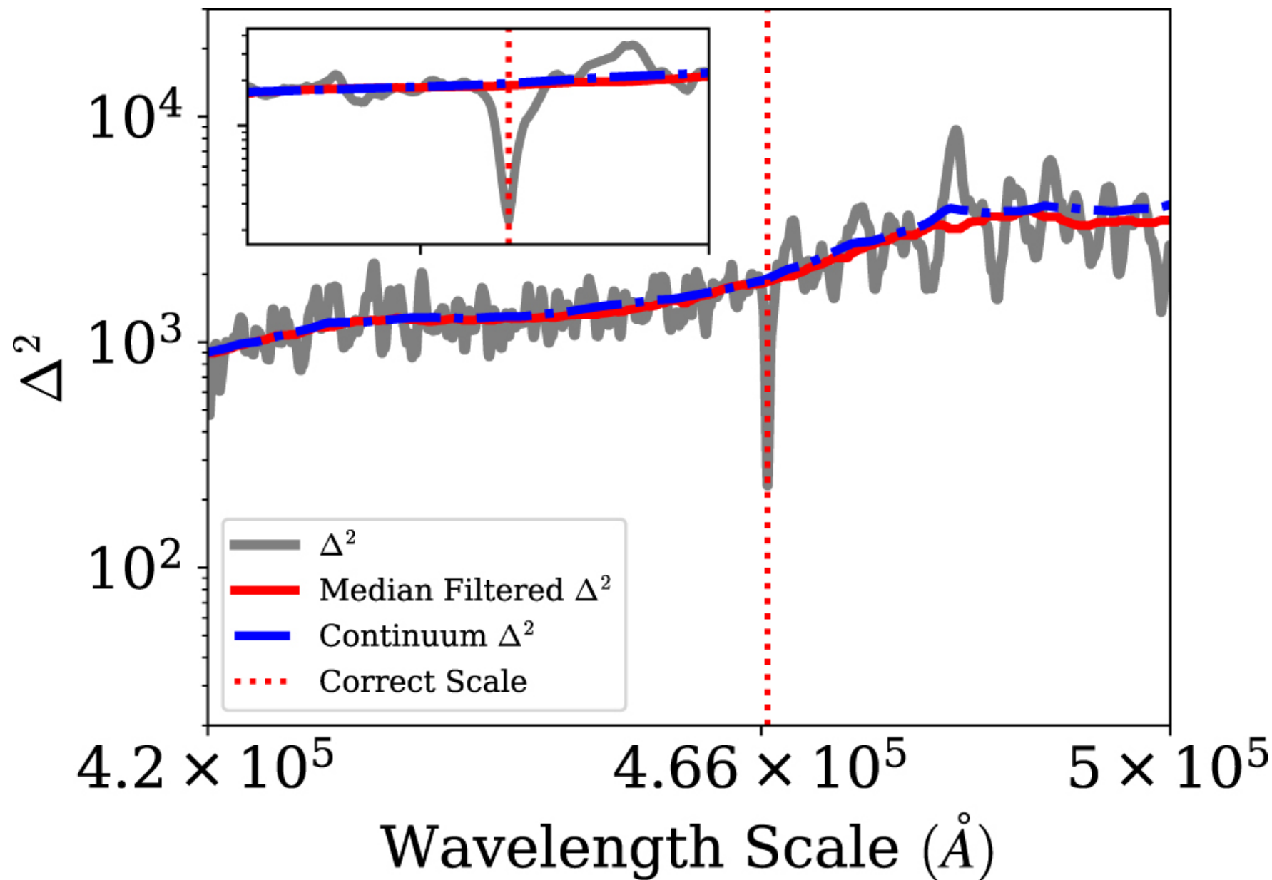
Figure B1. from Automatic Échelle Spectrograph Wavelength Calibration null 2020 AJ 160 25 doi:10.3847/1538-3881/ab929c https://dx.doi.org/10.3847/1538-3881/ab929c © 2020. The American Astronomical Society. All rights reserved.
