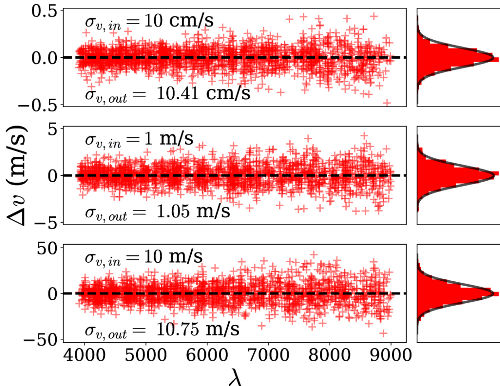
Figure 6. from Automatic Échelle Spectrograph Wavelength Calibration null 2020 AJ 160 25 doi:10.3847/1538-3881/ab929c https://dx.doi.org/10.3847/1538-3881/ab929c © 2020. The American Astronomical Society. All rights reserved.
