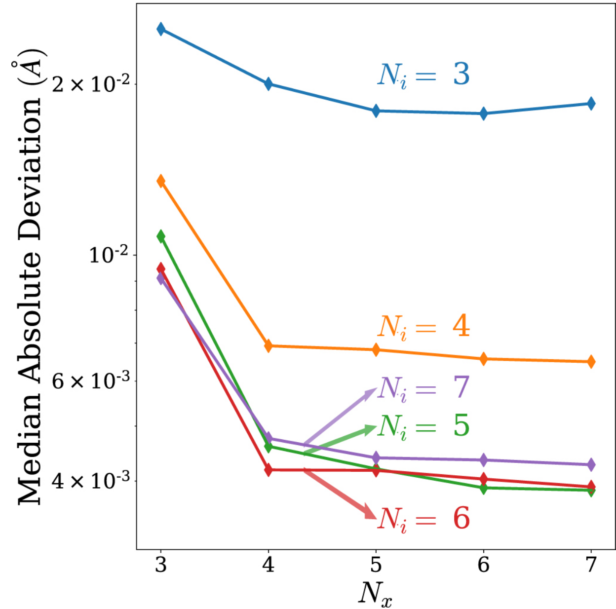
Figure 4. from Automatic Échelle Spectrograph Wavelength Calibration null 2020 AJ 160 25 doi:10.3847/1538-3881/ab929c https://dx.doi.org/10.3847/1538-3881/ab929c © 2020. The American Astronomical Society. All rights reserved.
