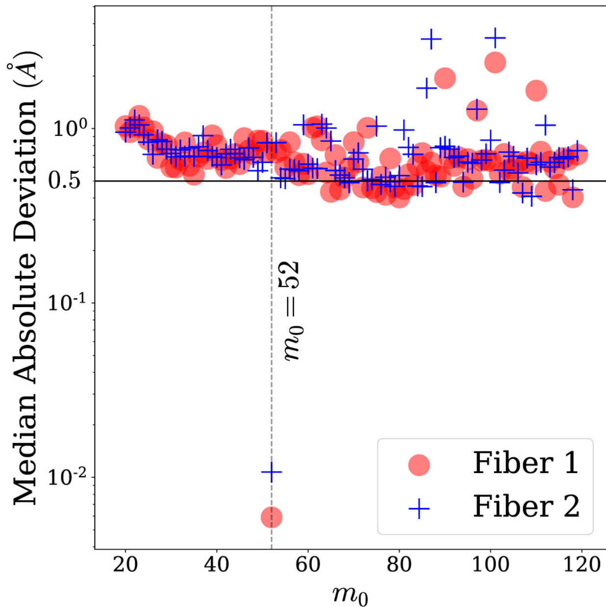
Figure 3. from Automatic Échelle Spectrograph Wavelength Calibration null 2020 AJ 160 25 doi:10.3847/1538-3881/ab929c https://dx.doi.org/10.3847/1538-3881/ab929c © 2020. The American Astronomical Society. All rights reserved.
