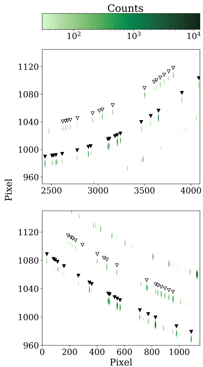
Figure 1. from Automatic Échelle Spectrograph Wavelength Calibration null 2020 AJ 160 25 doi:10.3847/1538-3881/ab929c https://dx.doi.org/10.3847/1538-3881/ab929c © 2020. The American Astronomical Society. All rights reserved.
