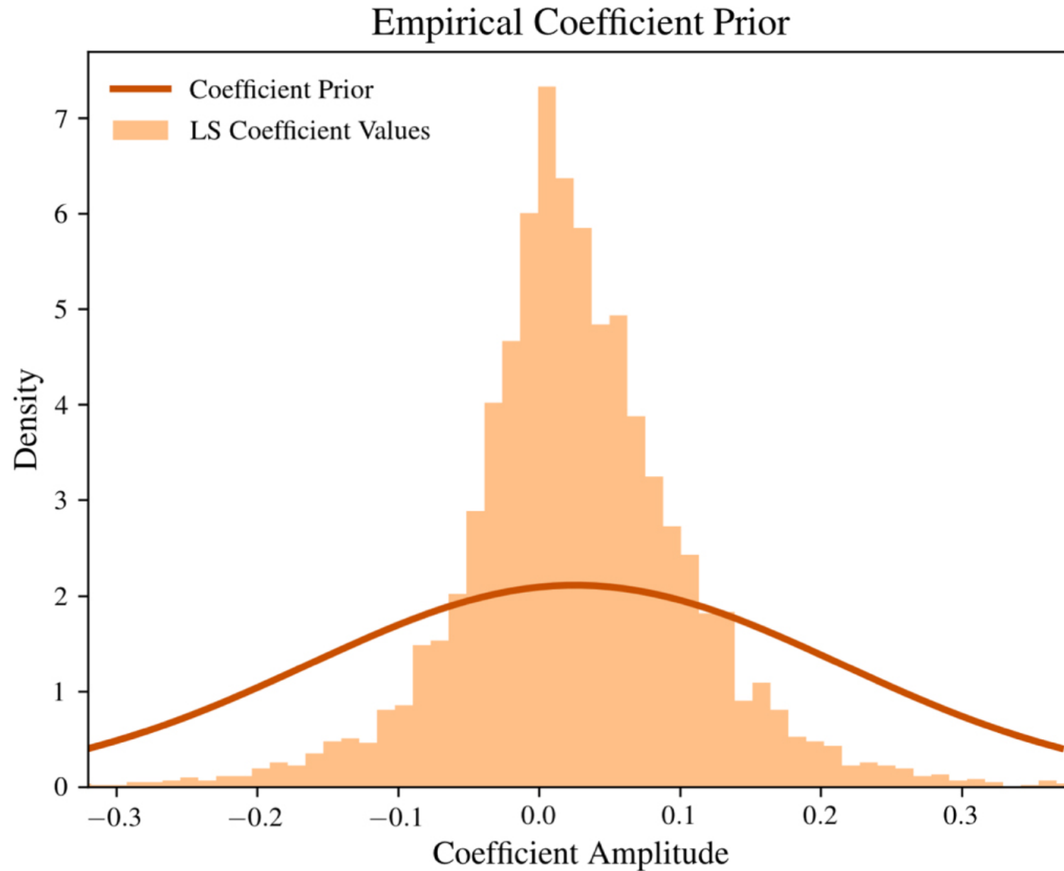
Figure 3. from Bayesian Methods for Joint Exoplanet Transit Detection and Systematic Noise Characterization null 2020 AJ 159 283 doi:10.3847/1538-3881/ab8e38 https://dx.doi.org/10.3847/1538-3881/ab8e38 © 2020. The American Astronomical Society. All rights reserved.
