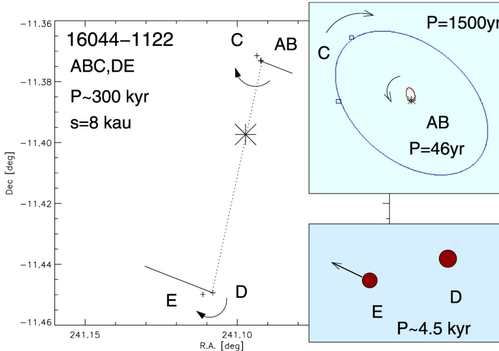
Figure 8. from Nearby Quintuple Systems Tucanae and Scorpii null 2020 AJ 159 265 doi:10.3847/1538-3881/ab8af1 https://dx.doi.org/10.3847/1538-3881/ab8af1 © 2020. The American Astronomical Society. All rights reserved.
