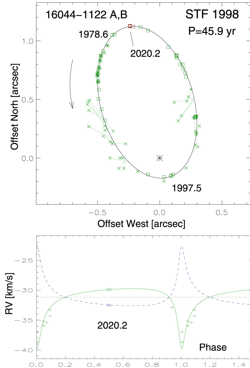
Figure 7. from Nearby Quintuple Systems Tucanae and Scorpii null 2020 AJ 159 265 doi:10.3847/1538-3881/ab8af1 https://dx.doi.org/10.3847/1538-3881/ab8af1 © 2020. The American Astronomical Society. All rights reserved.
