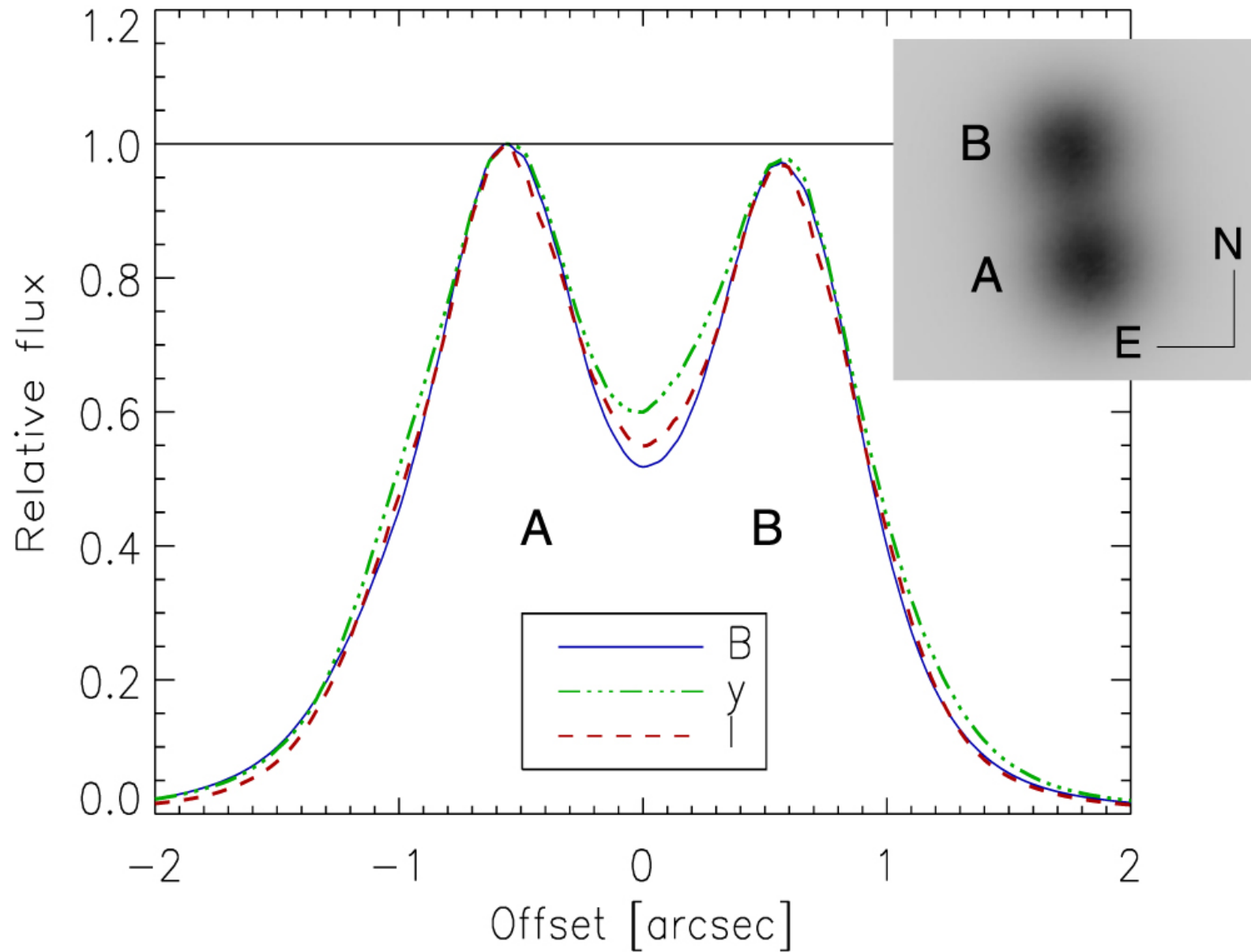
Figure 6. from Nearby Quintuple Systems Tucanae and Scorpii null 2020 AJ 159 265 doi:10.3847/1538-3881/ab8af1 https://dx.doi.org/10.3847/1538-3881/ab8af1 © 2020. The American Astronomical Society. All rights reserved.
